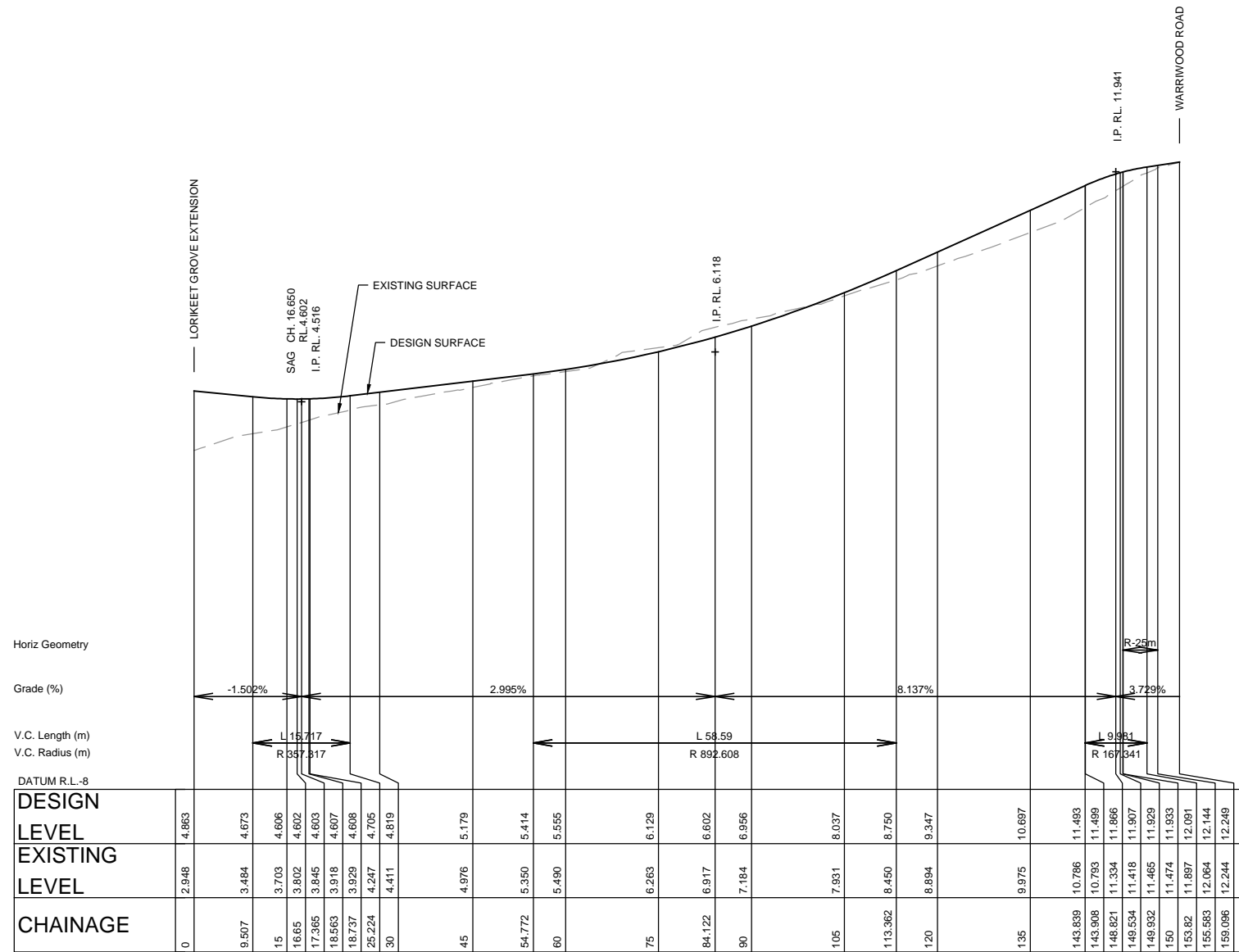
LONGITUDINAL SECTION - ROAD No.1 HORIZONTAL SCALE - 1:500 VERTICAL SCALE - 1:100
