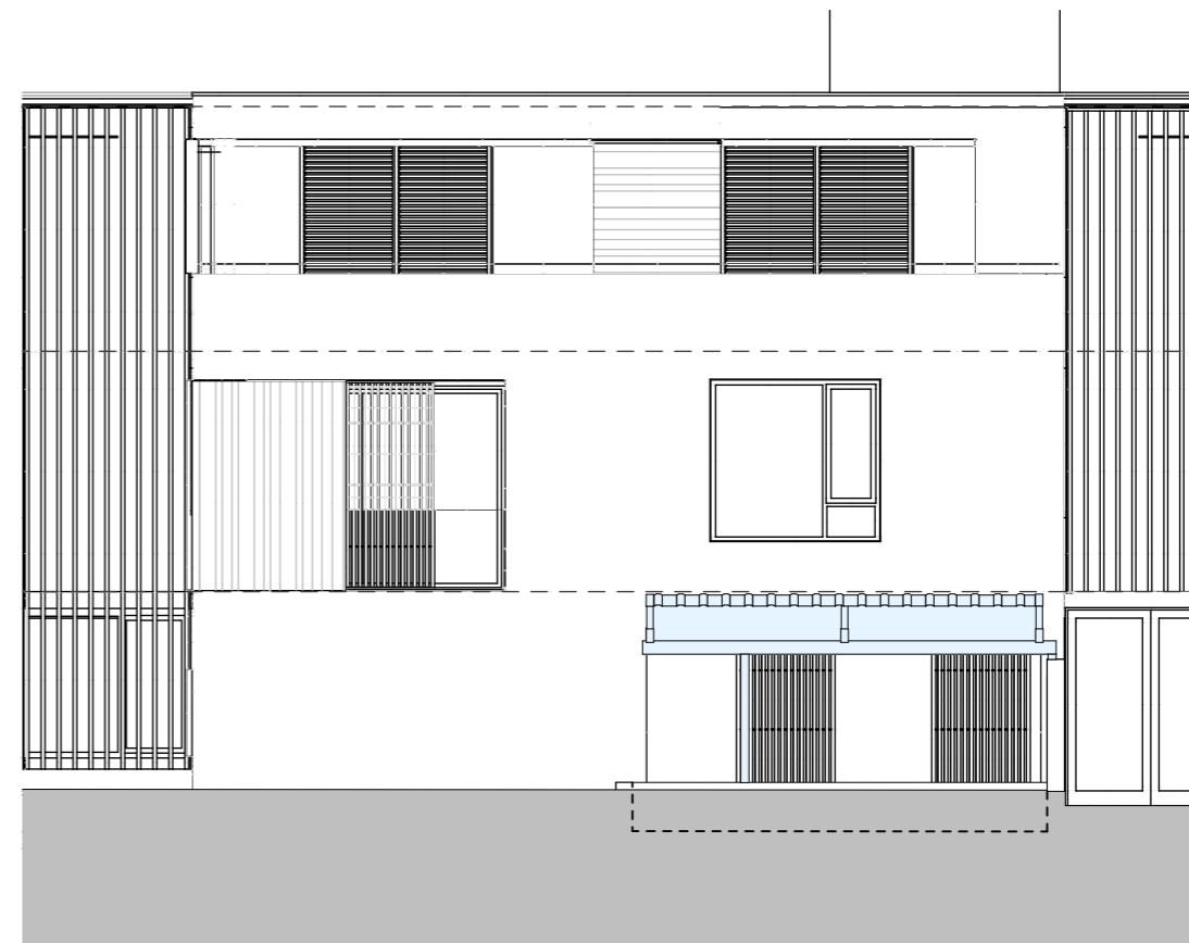
2 - Typical Elevation - Building A & B 1:100
