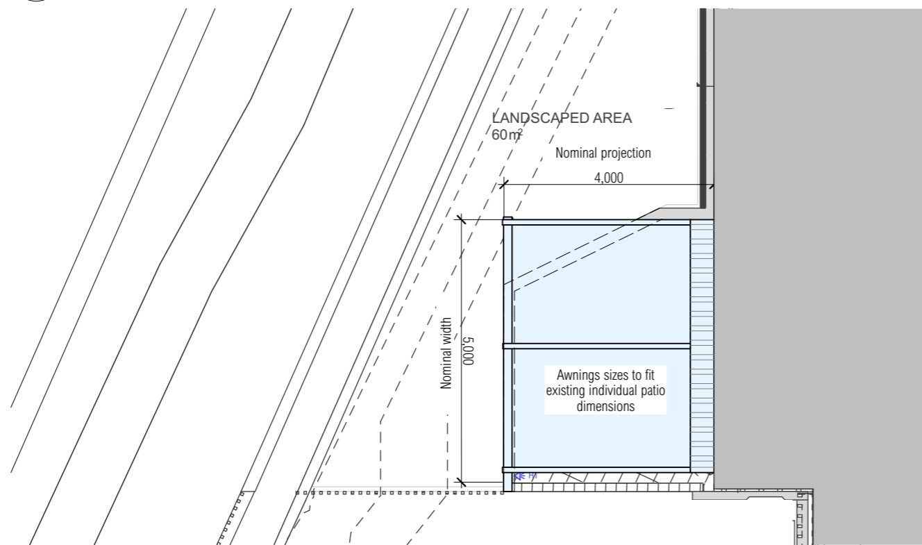
3 - Typical Plan - Building A & B 1:100
