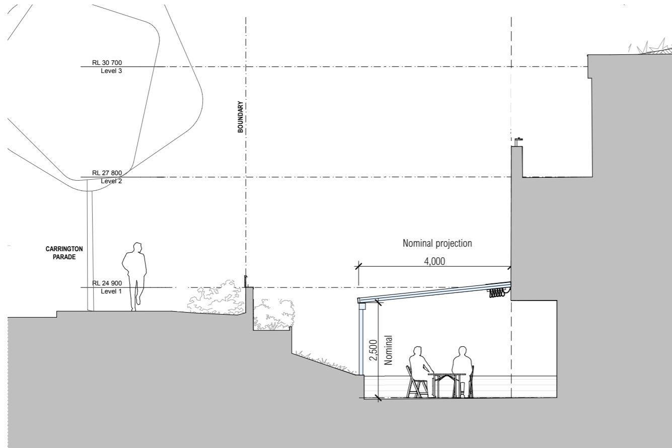
1 - Typical Section - Building A & B 1:100
