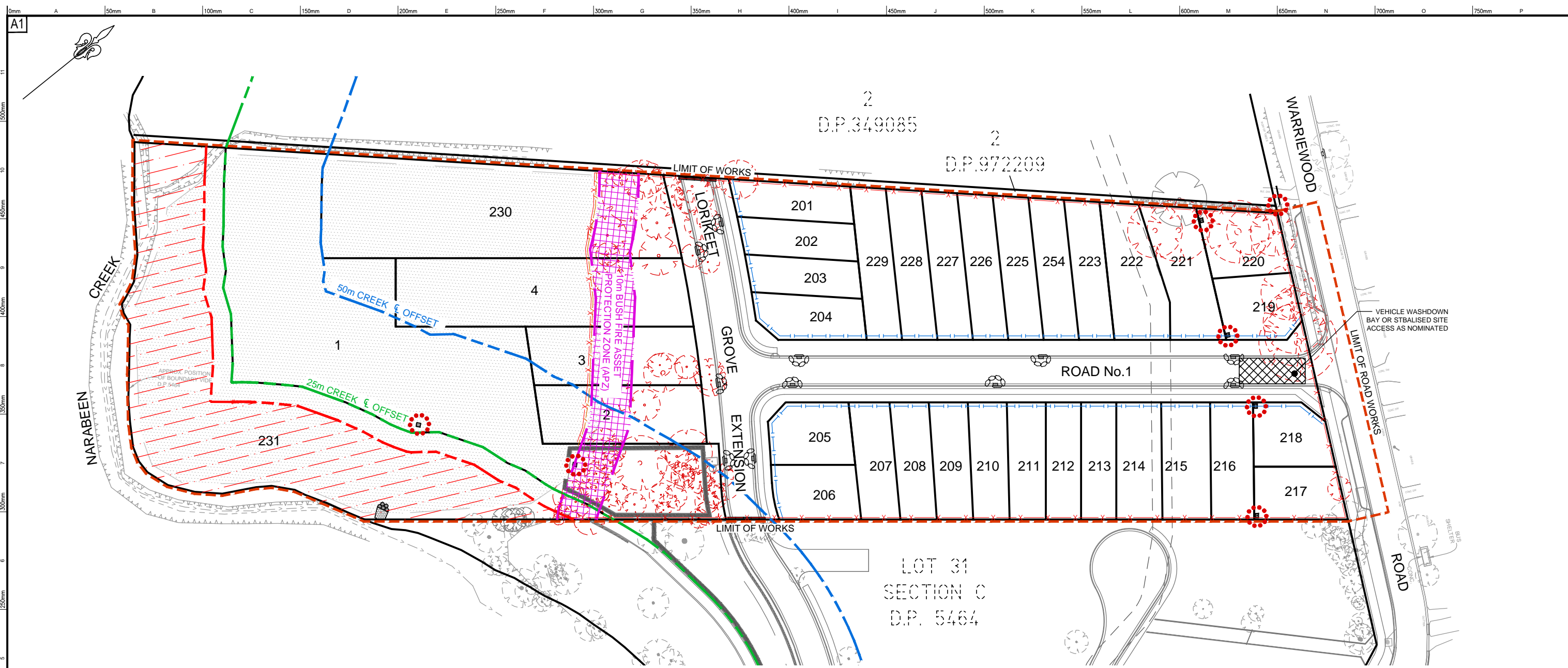
PLAN 1:500
