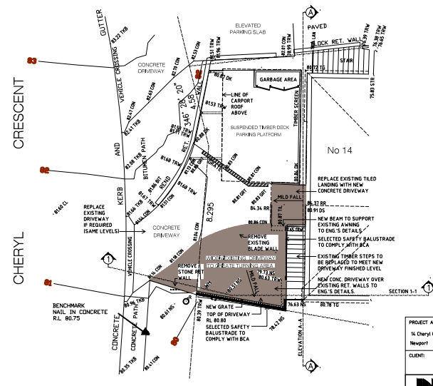
PROPOSED DRIVEWAY LAYOUT
