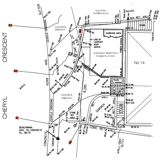
EXISTING CARPORT / DRIVEWAY LAYOUT
