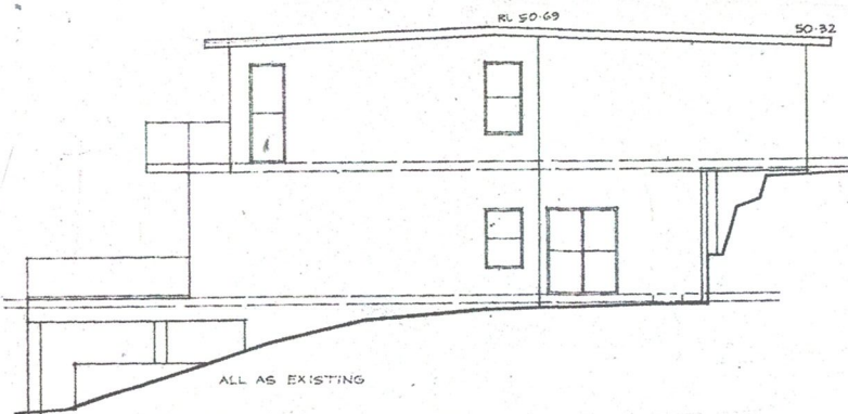
NORTHWEST ELEVATION
