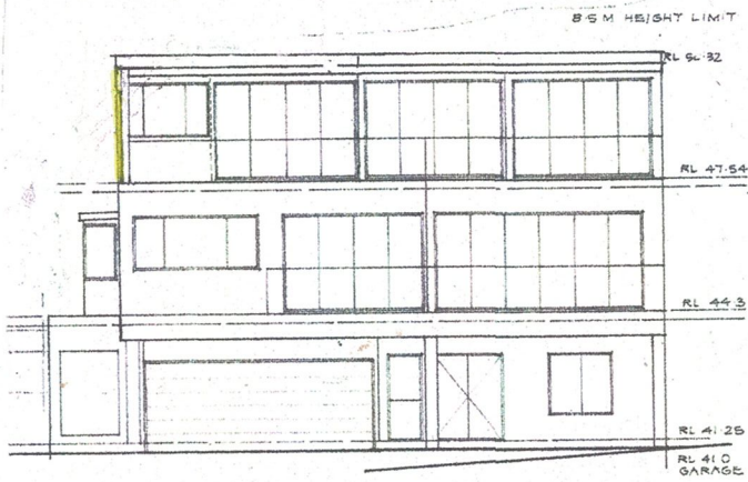
NORTHEAST ELEVATION
