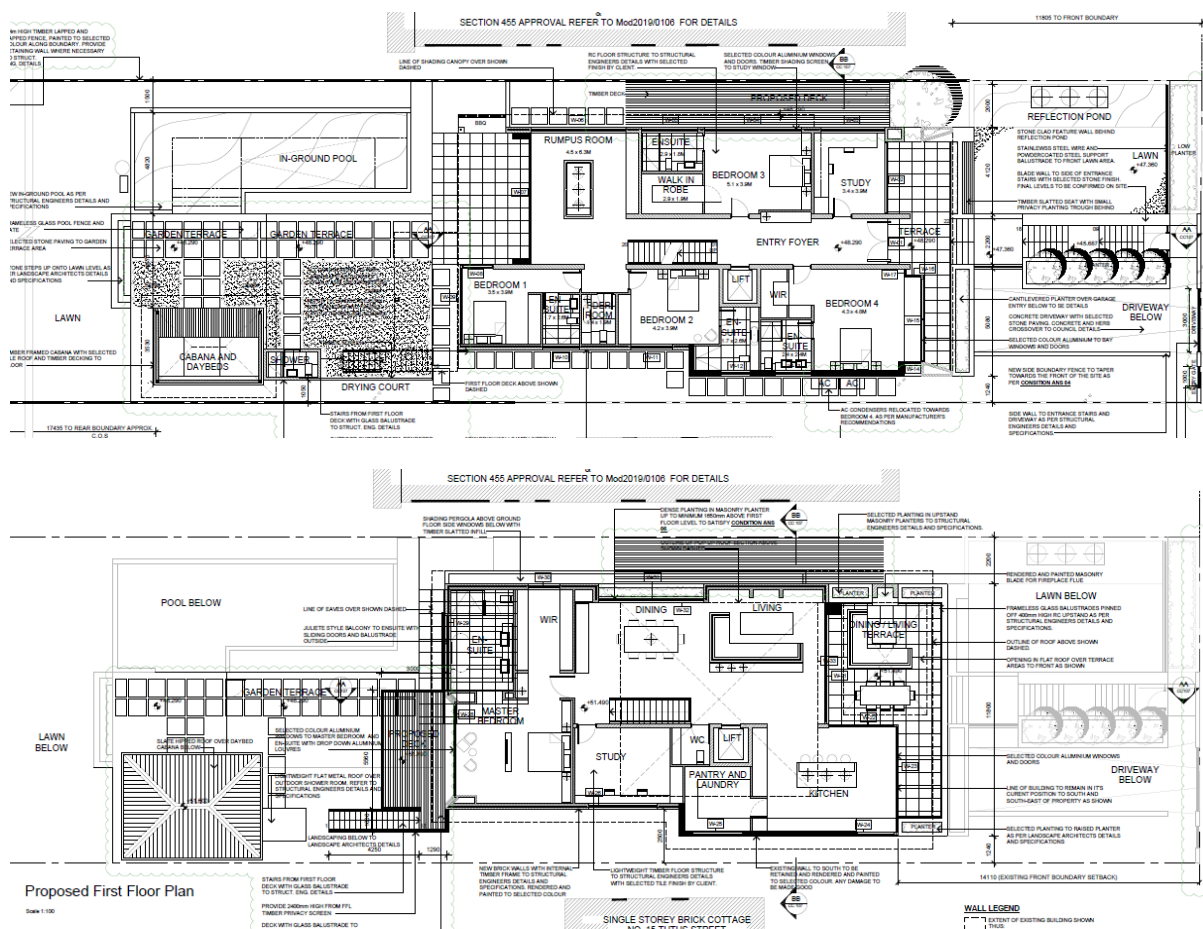
Figure 2: Floor plans.
