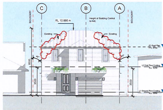
4 Proposed Elevation 3 - a 1:100
