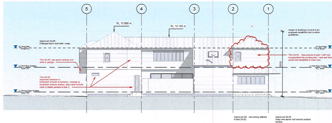
2 Proposed Elevation 1 - a 1:100
