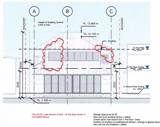
4 Proposed Elevation 4 - a 1 : 100
