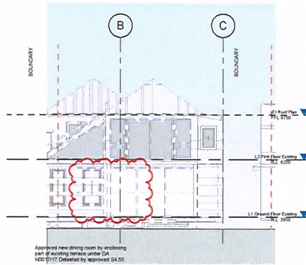
3 Existing Elevation 4 - a 1 : 100
