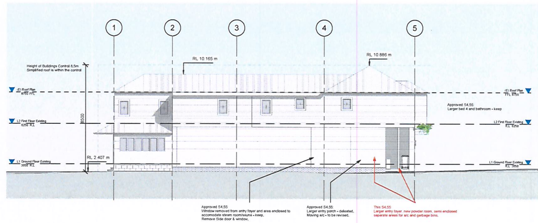
2 Proposed Elevation 2 - a 1 : 100
