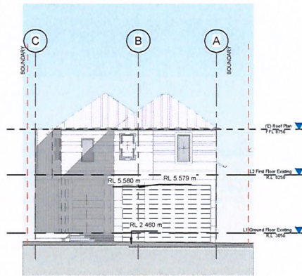
3 Existing Elevation 3 - a 1:100
