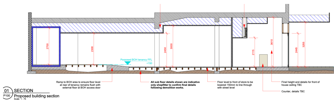
Figure 3. Proposed Building Section Source: Craveable Brands
