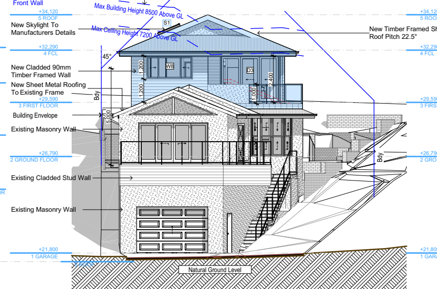
E-03 South 1:200
