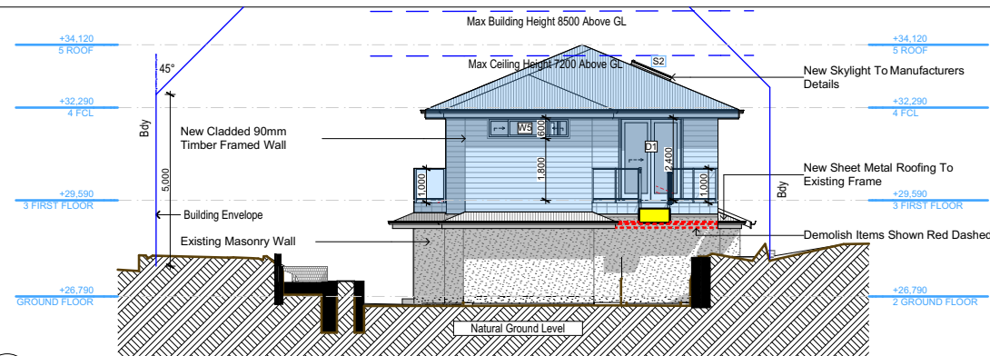
E-01 North 1:200
