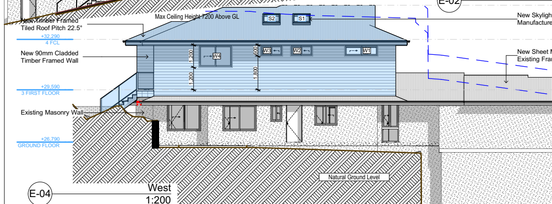
E-02 East 1:200
