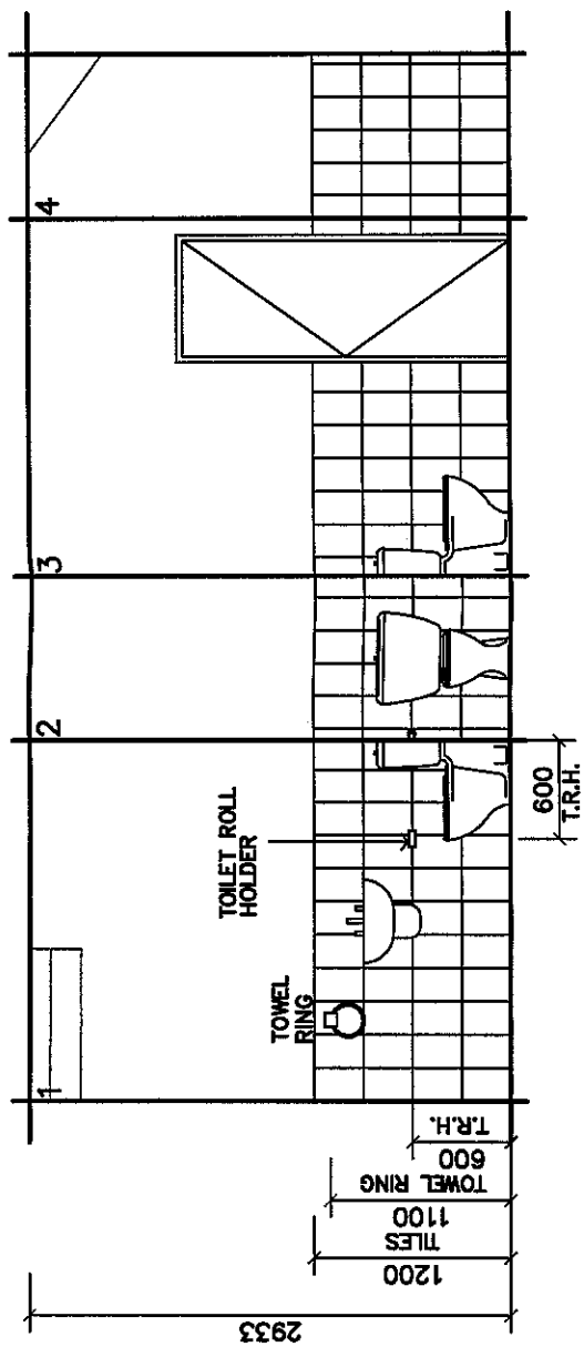
W.C. DETAIL
