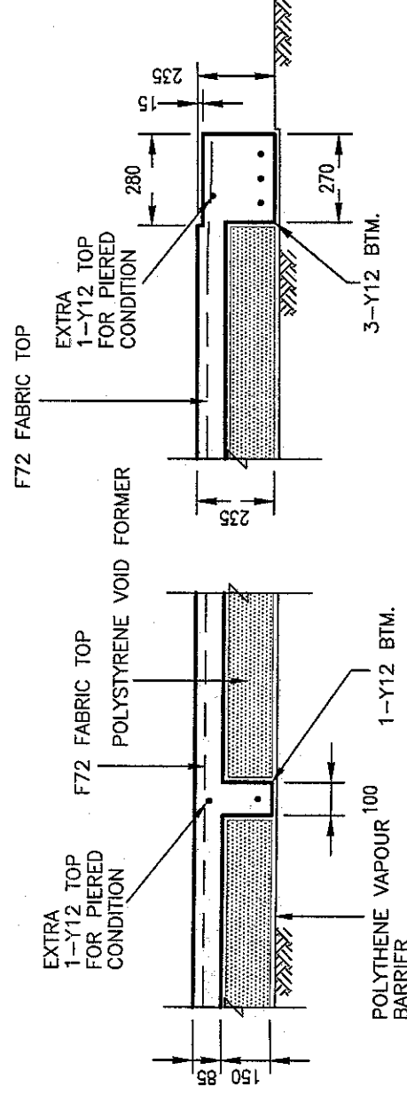
INTERNAL RIB
