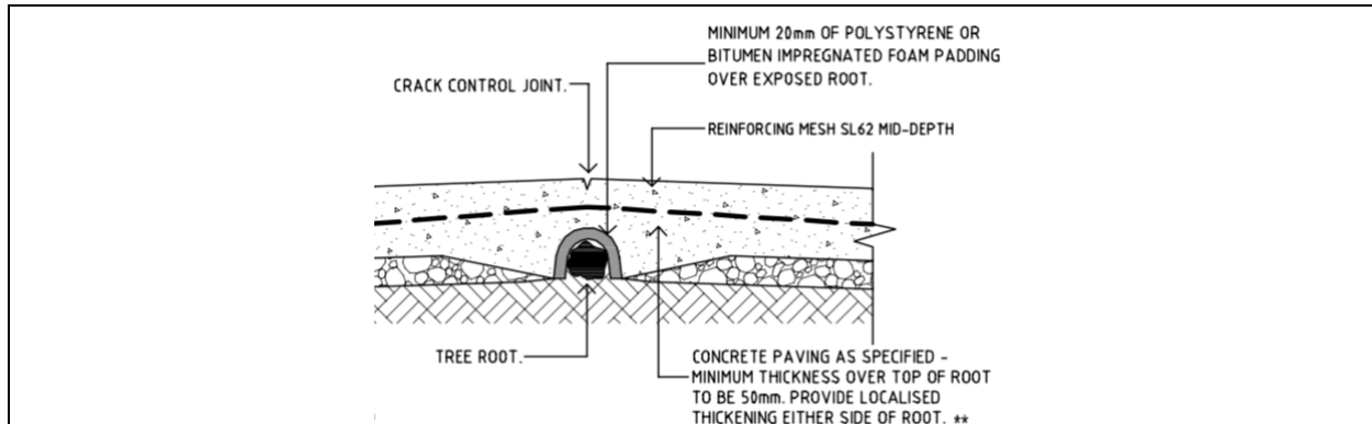
Image D: Example method for bridging concrete surfacing over tree roots provided in the Canterbury Bankstown Council standard drawings. 7
