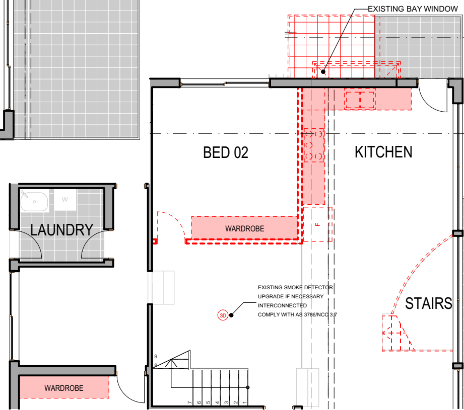
FIRST FLOOR DEMOLITION PLAN - 1:100
