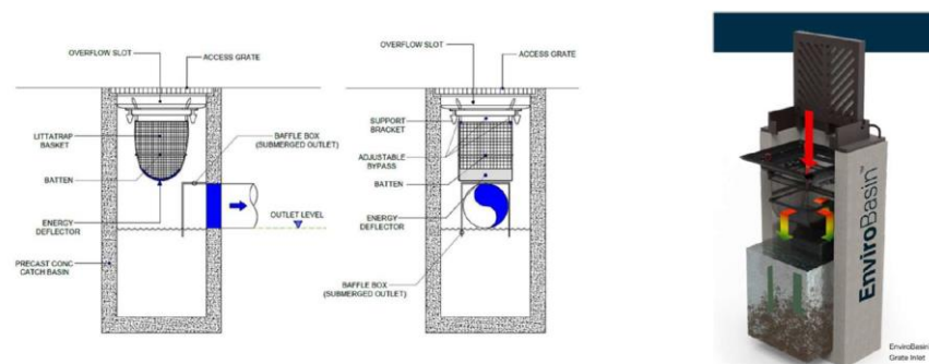
Figure 5. 1 EnviroBasin Detail
