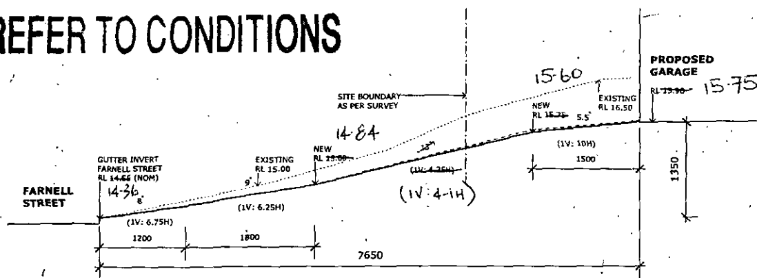
DRIVEWAY SECTION X-X SCALE 1:50
