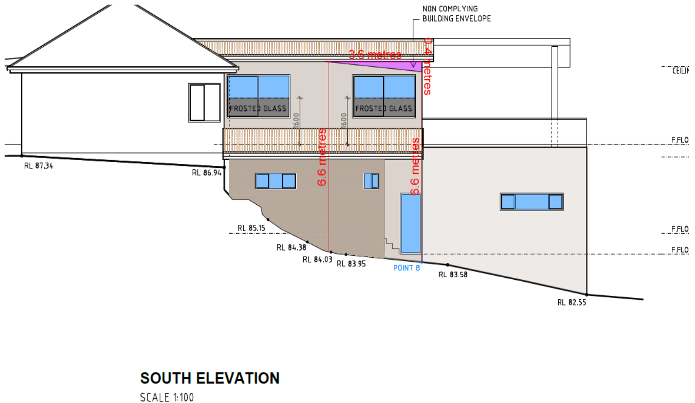
Figure 1: Envelope non-compliance (southern elevation)
