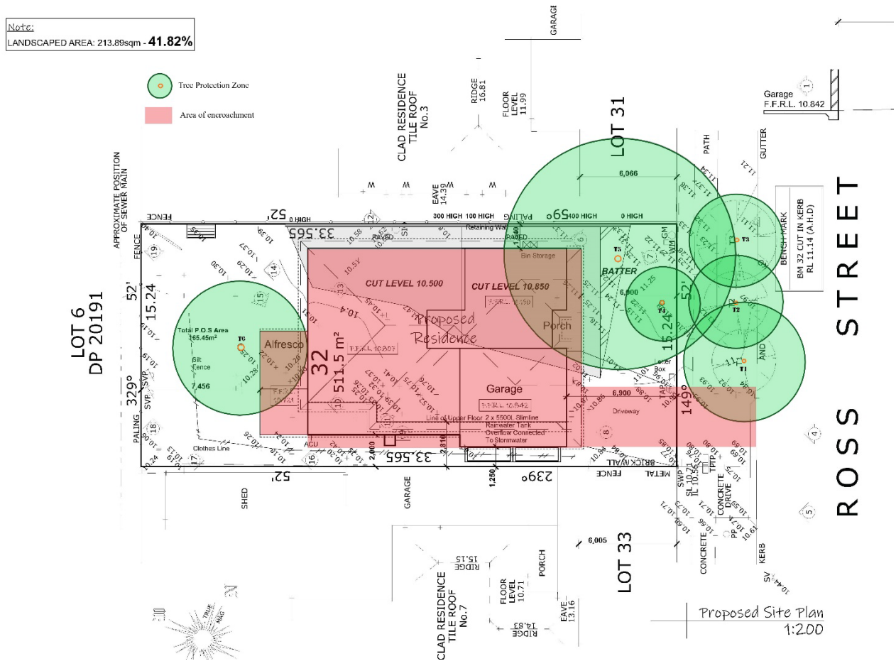
Figure 3: TPZ Plan
