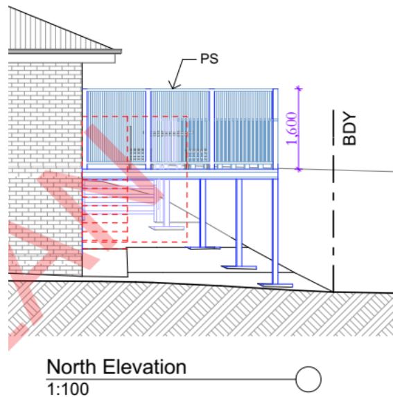
Figure 2: Elevation showing the proposed decking located upon piers. (Northern Beaches Designs 19/05/2025)
