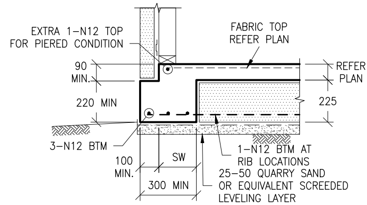
TYPICAL EDGE BEAM DETAIL
