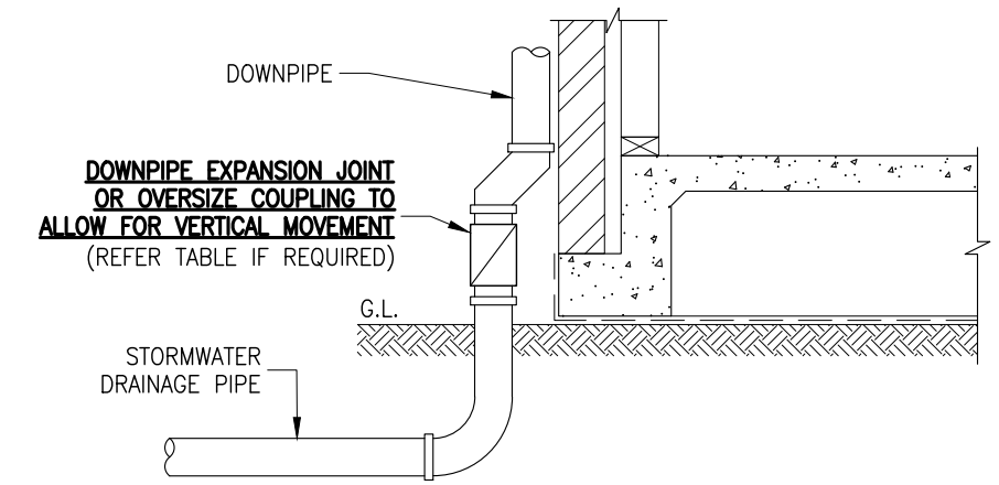
TYPICAL STORMWATER DETAIL (ELEVATION VIEW)
