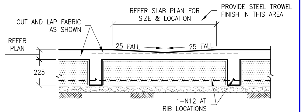
TYPICAL SHOWER AREA DETAIL
