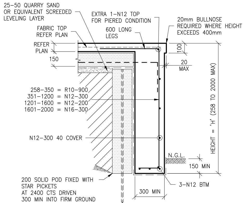
TYPICAL DEEPENED PATIO EDGE BEAM DETAIL
