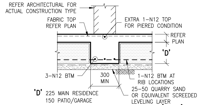
INTERNAL BEAM DETAIL - 'IB1'
