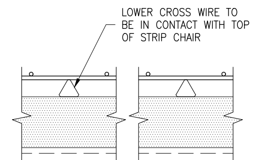
TYPICAL CHAIR DETAIL
