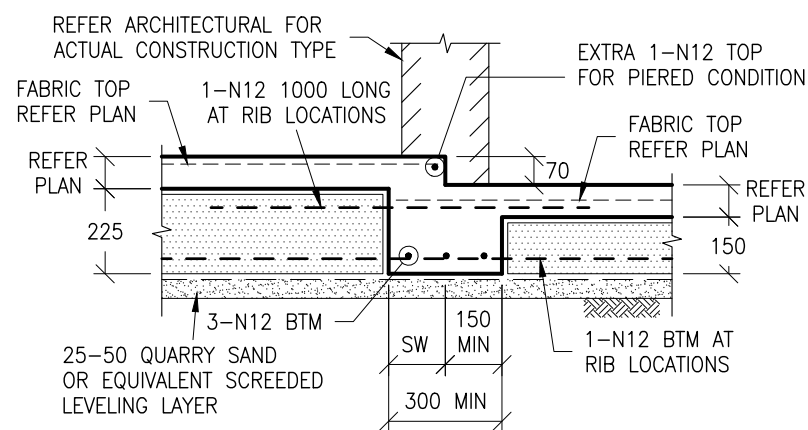
TYPICAL PATIO STEP BEAM DETAIL
