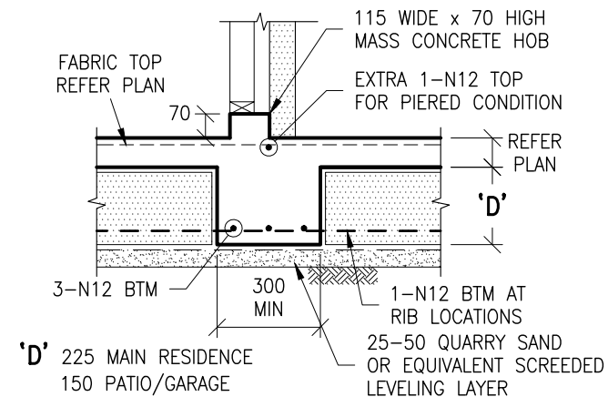
TYPICAL INTERNAL BEAM DETAIL
