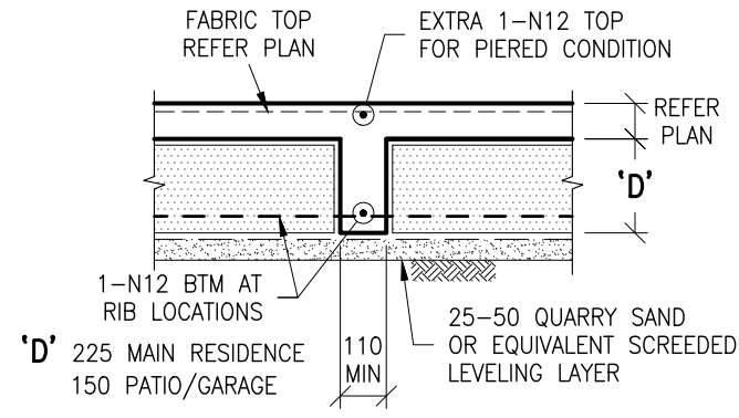
TYPICAL RIB BEAM DETAIL
