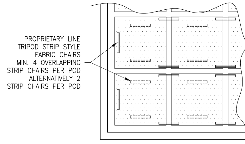
PLAN VIEW OF FABRIC CHAIR ORIENTATION
