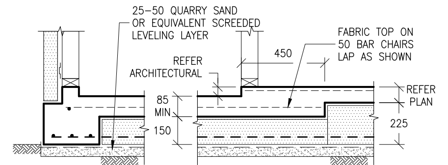
TYPICAL WET AREA RECESS DETAIL TO BE USED IN ACCORDANCE WITH THE ARCHITECTURAL
