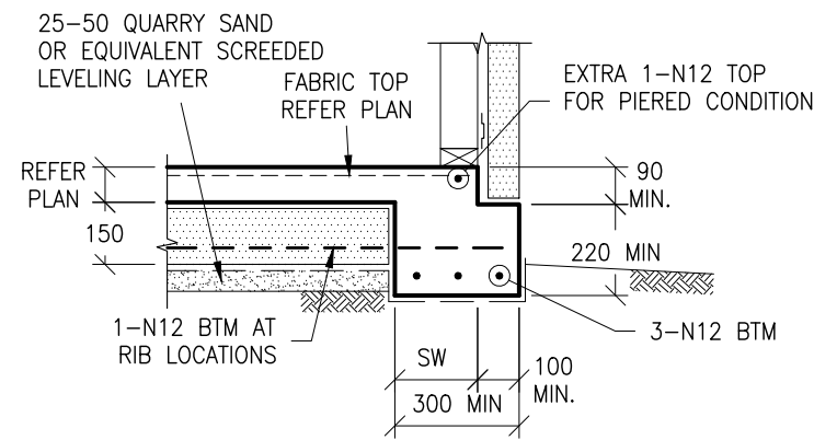
TYPICAL GARAGE EDGE BEAM DETAIL
