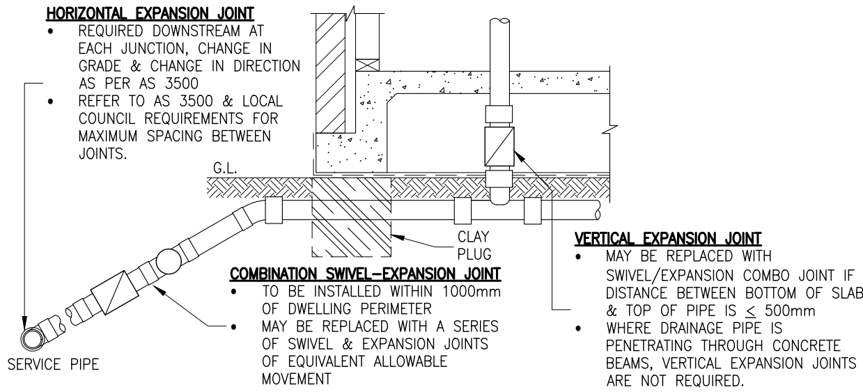
TYP. UNDER SLAB EDGE DETAIL (ELEVATION VIEW)
