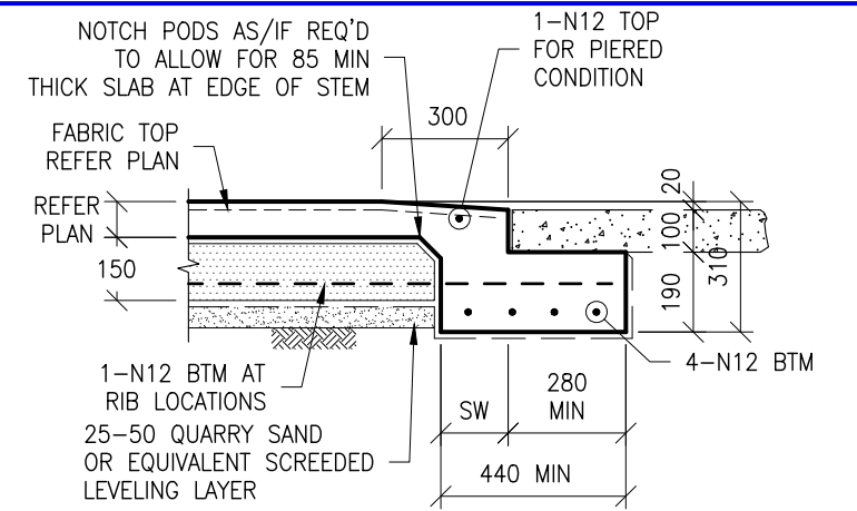
TYPICAL GARAGE DOOR REBATE DETAIL
