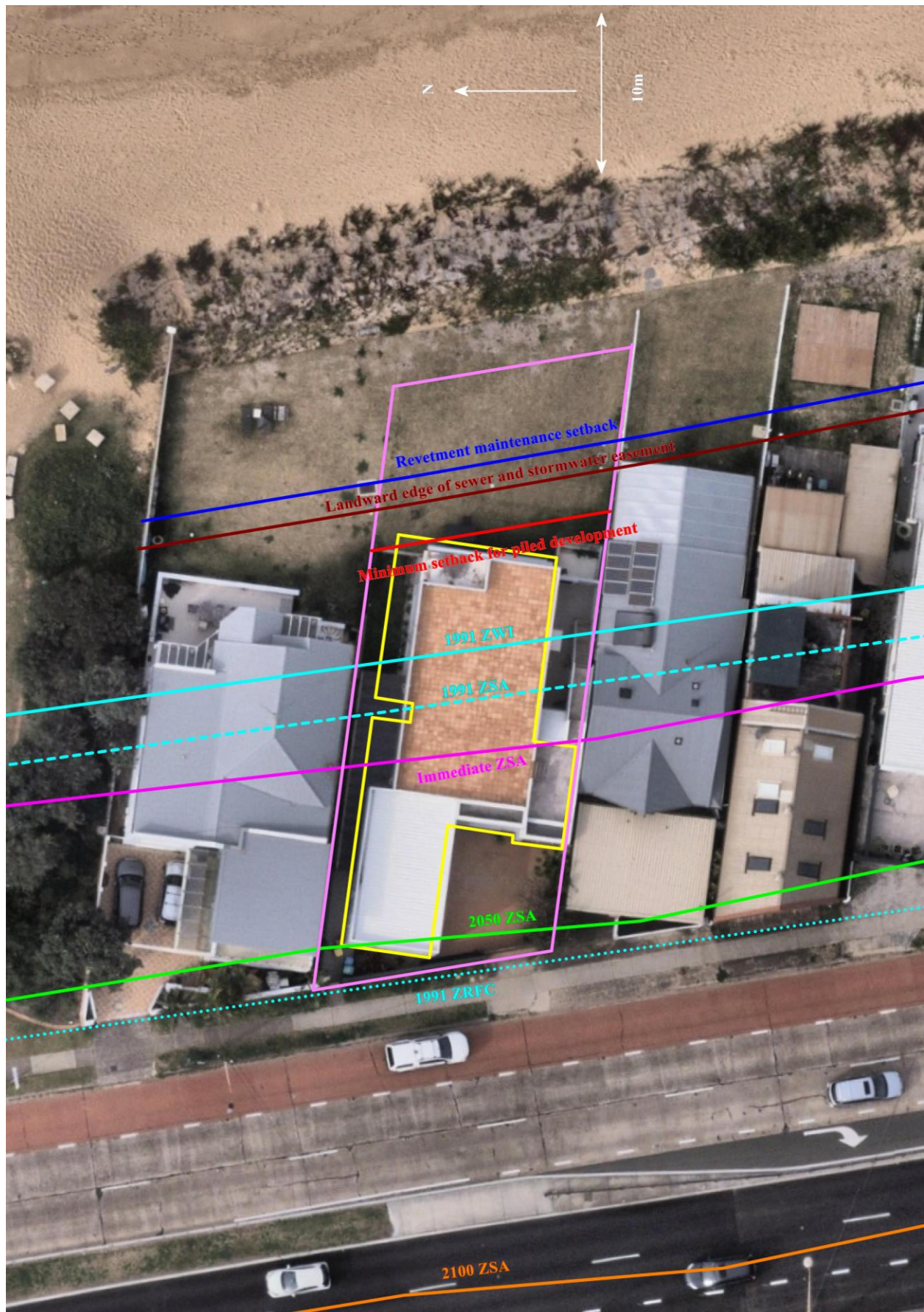
Figure 5: Coastal hazard lines and CZMP setbacks at site, with proposed dwelling outline in yellow, surveyed boundary in pink, and aerial photograph taken on 22 July 2024
