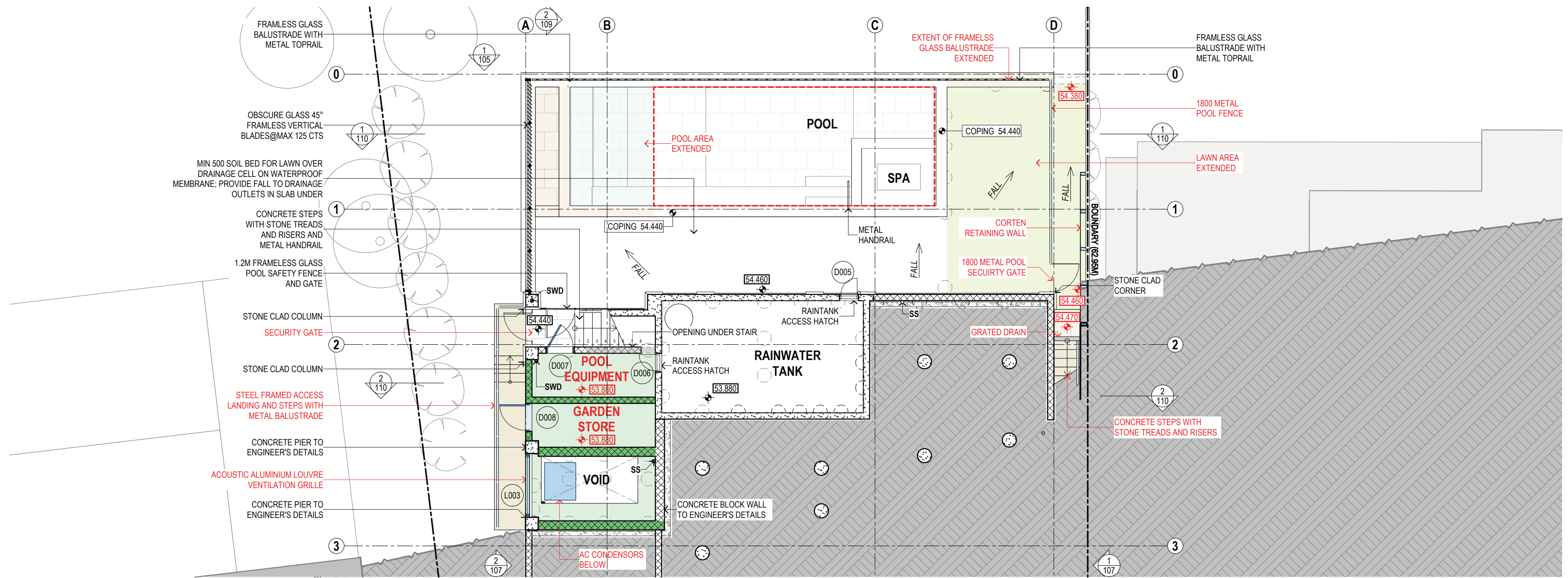
POOL LEVEL 1:100
