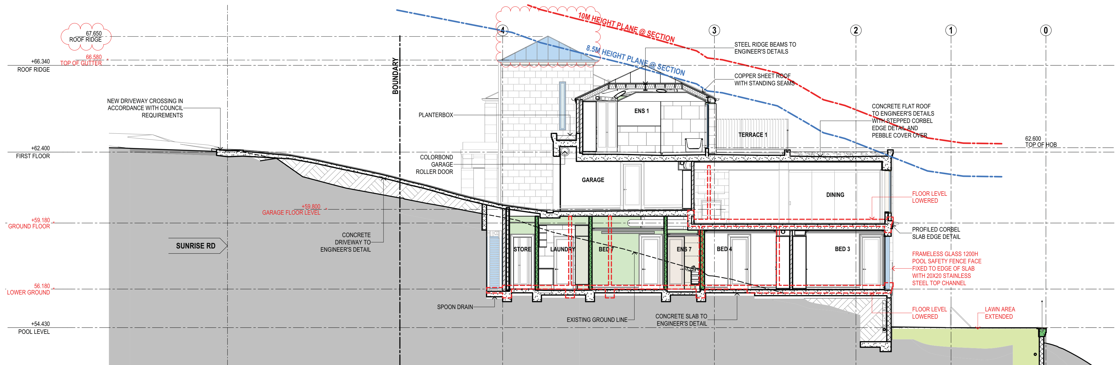
SECTION 1:100
