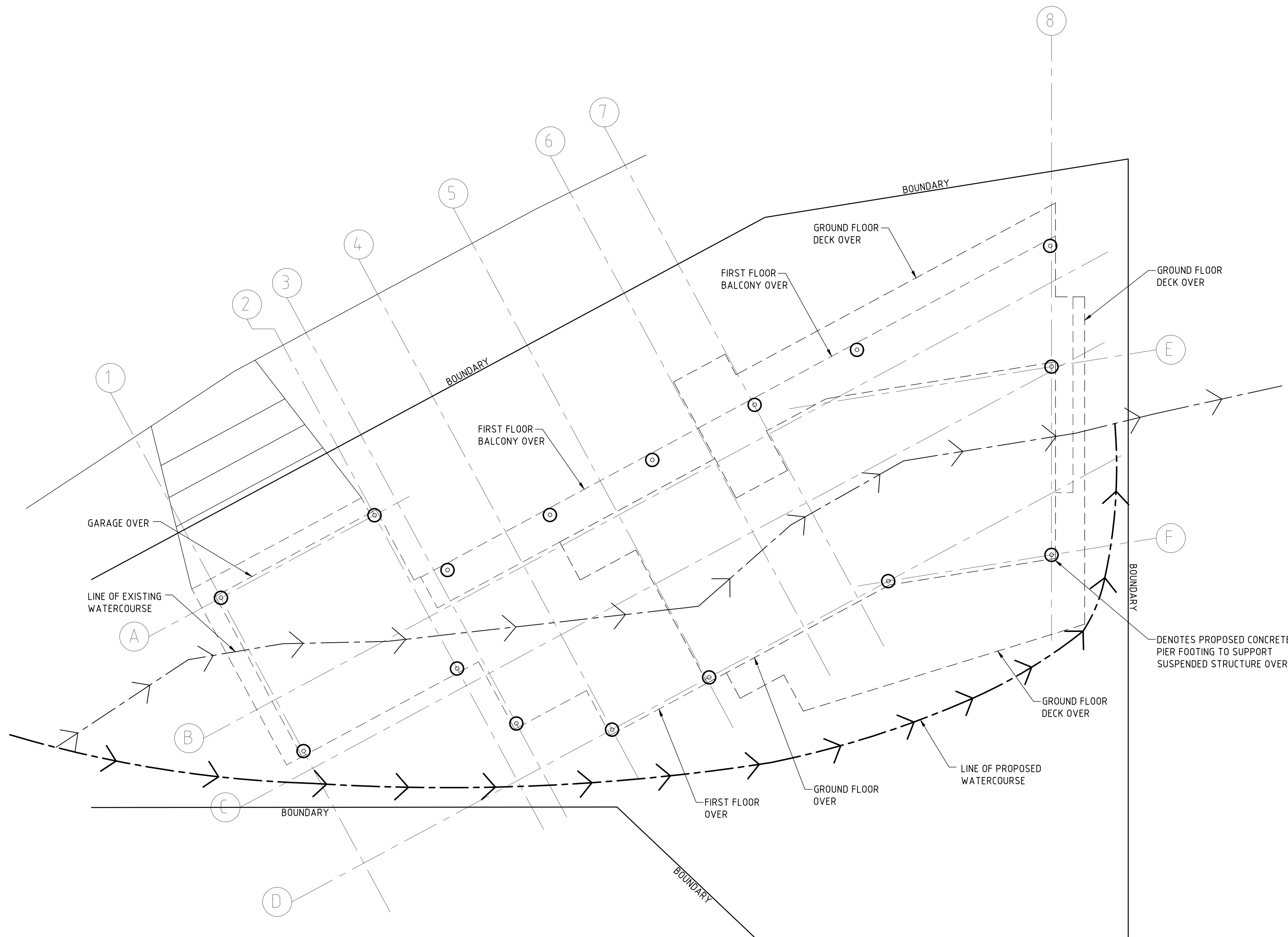
FOOTING PLAN SCALE 1:100
