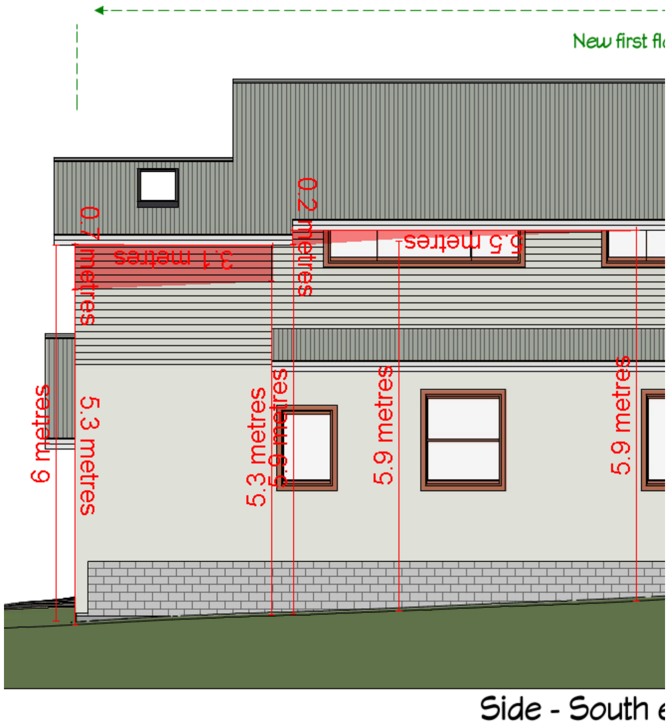
Figure 1: Side- South Elevation (depicting envelope non-compliance)
