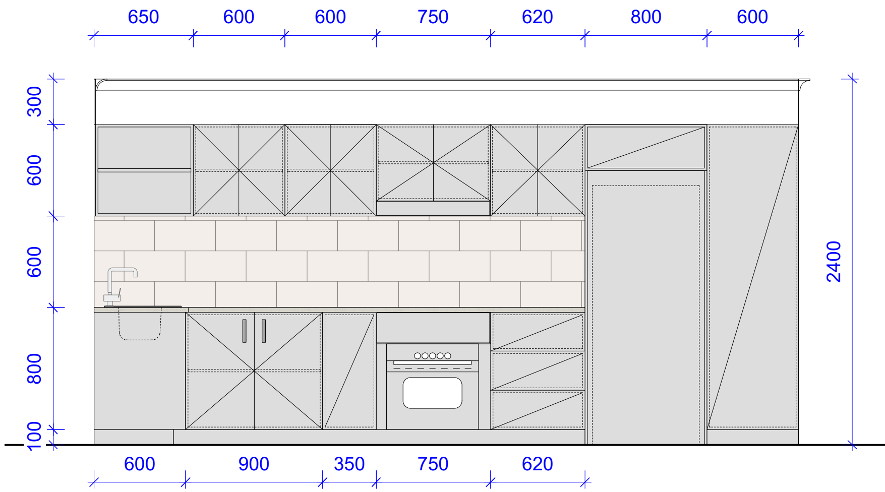
Elevation A 1:25@A1 1:50@A3. Do not scale off plan
