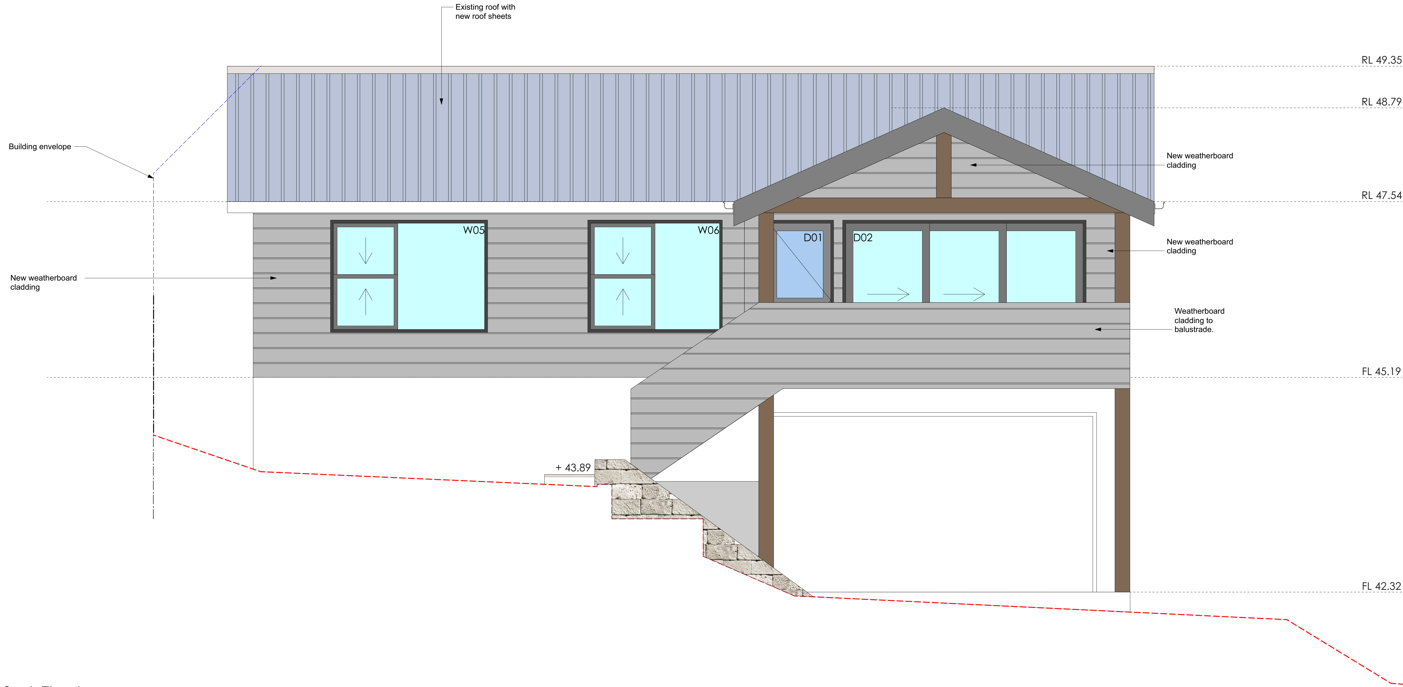
South Elevation 1:25@A1 1:50@A3. Do not scale off plan
