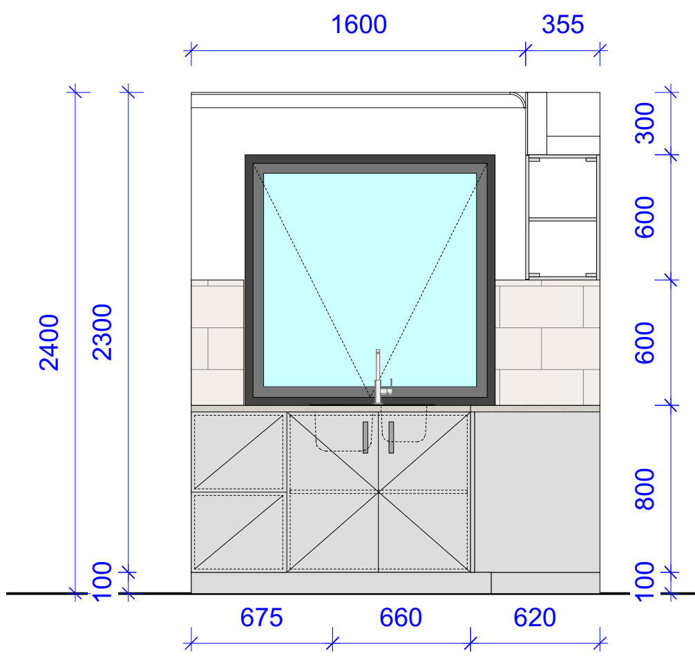
Elevation B 1:25@A1 1:50@A3. Do not scale off plan
