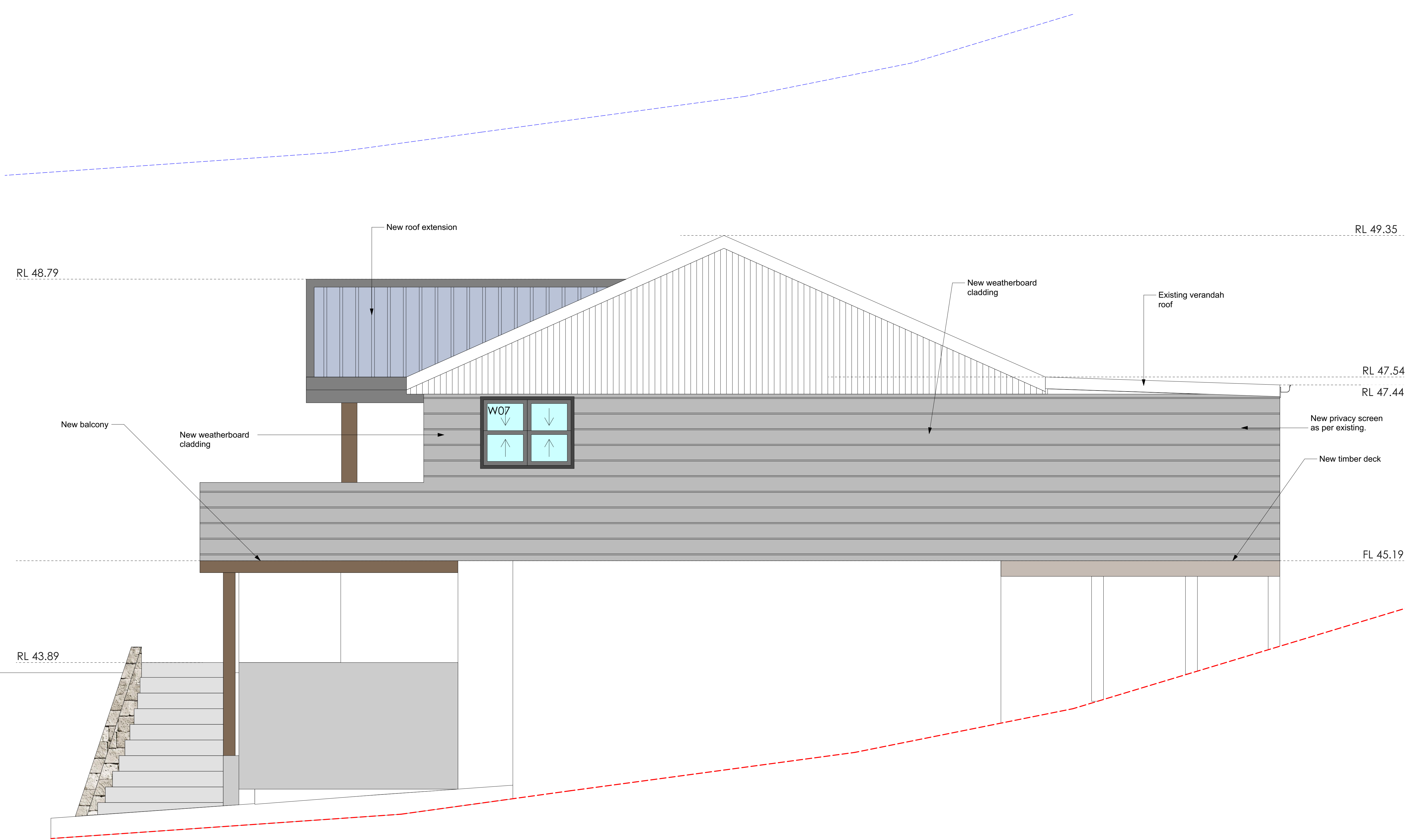
East Elevation 1:25@A1 1:50@A3. Do not scale off plan
