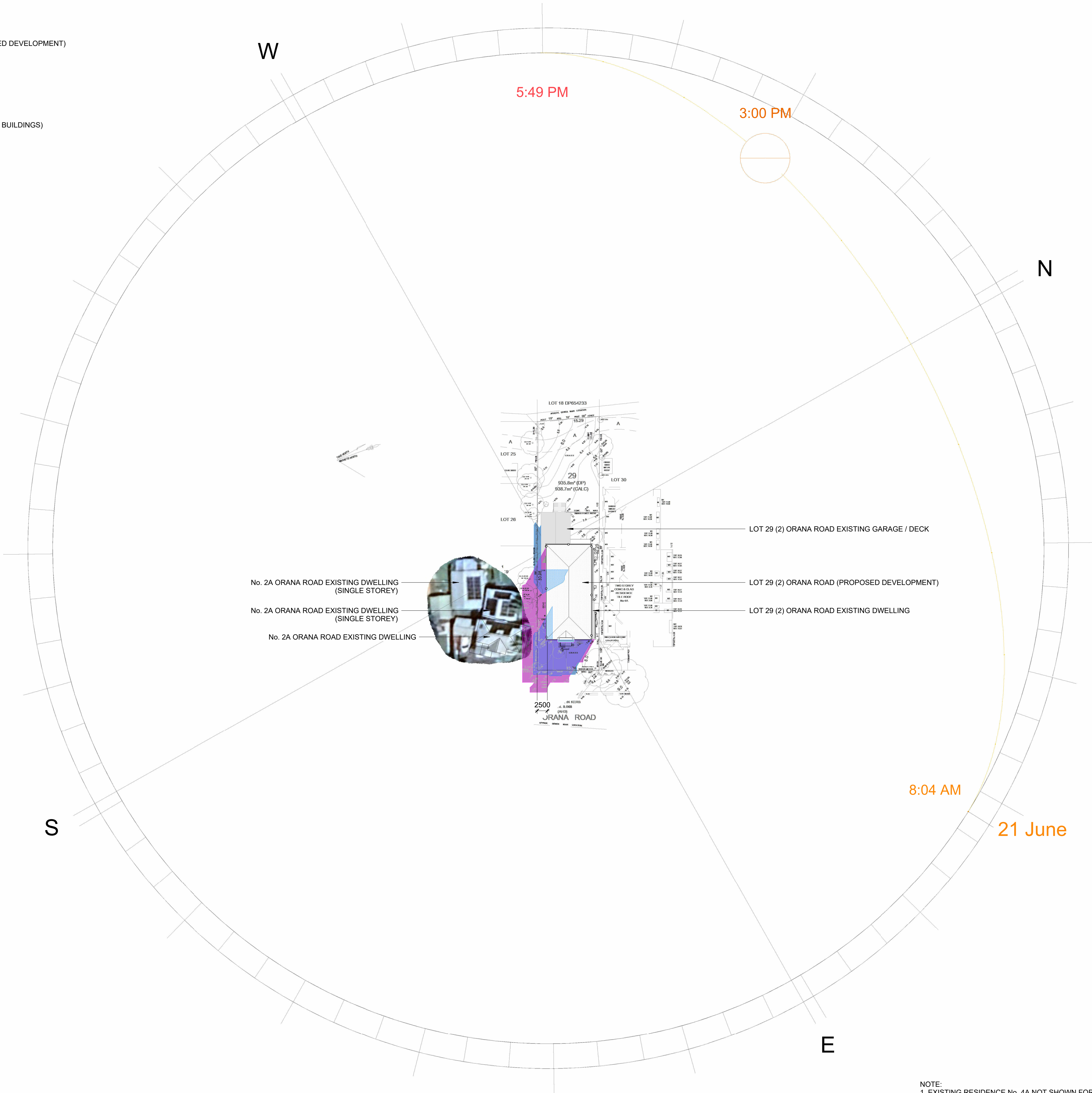
3pm 21ST JUNE SUN SHADOW DIAGRAM scale 1:500
