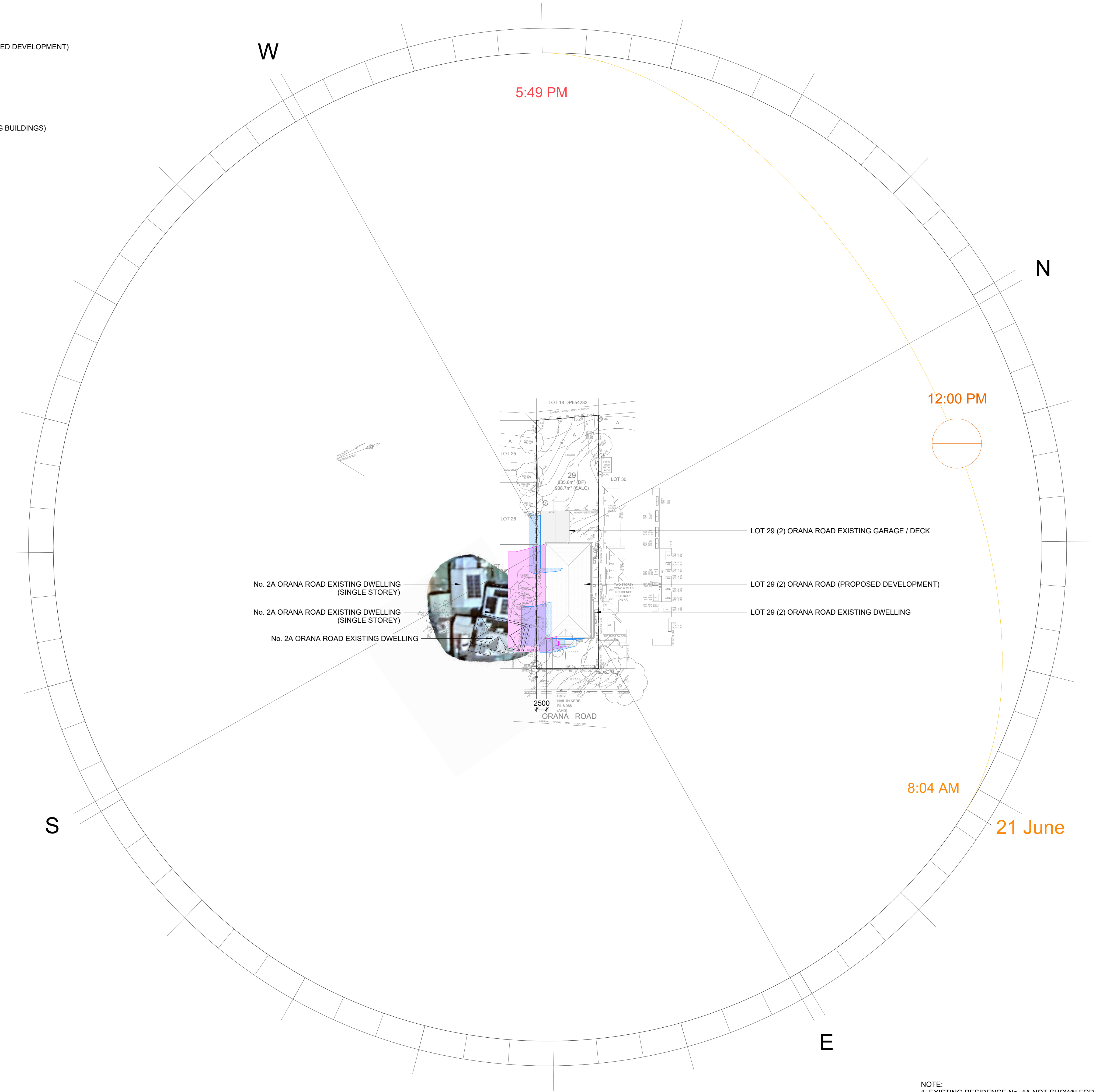
12pm 21ST JUNE SUN SHADOW DIAGRAM scale 1:500
