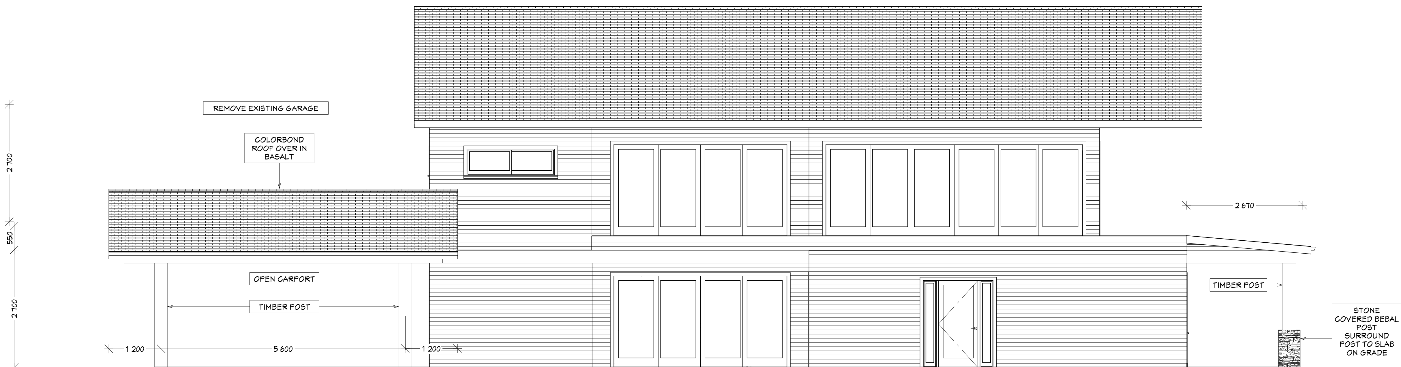
EAST ELEVATION 1:50
