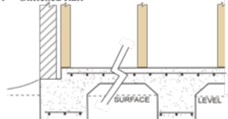
Fig. 1 Stiffened Raft
