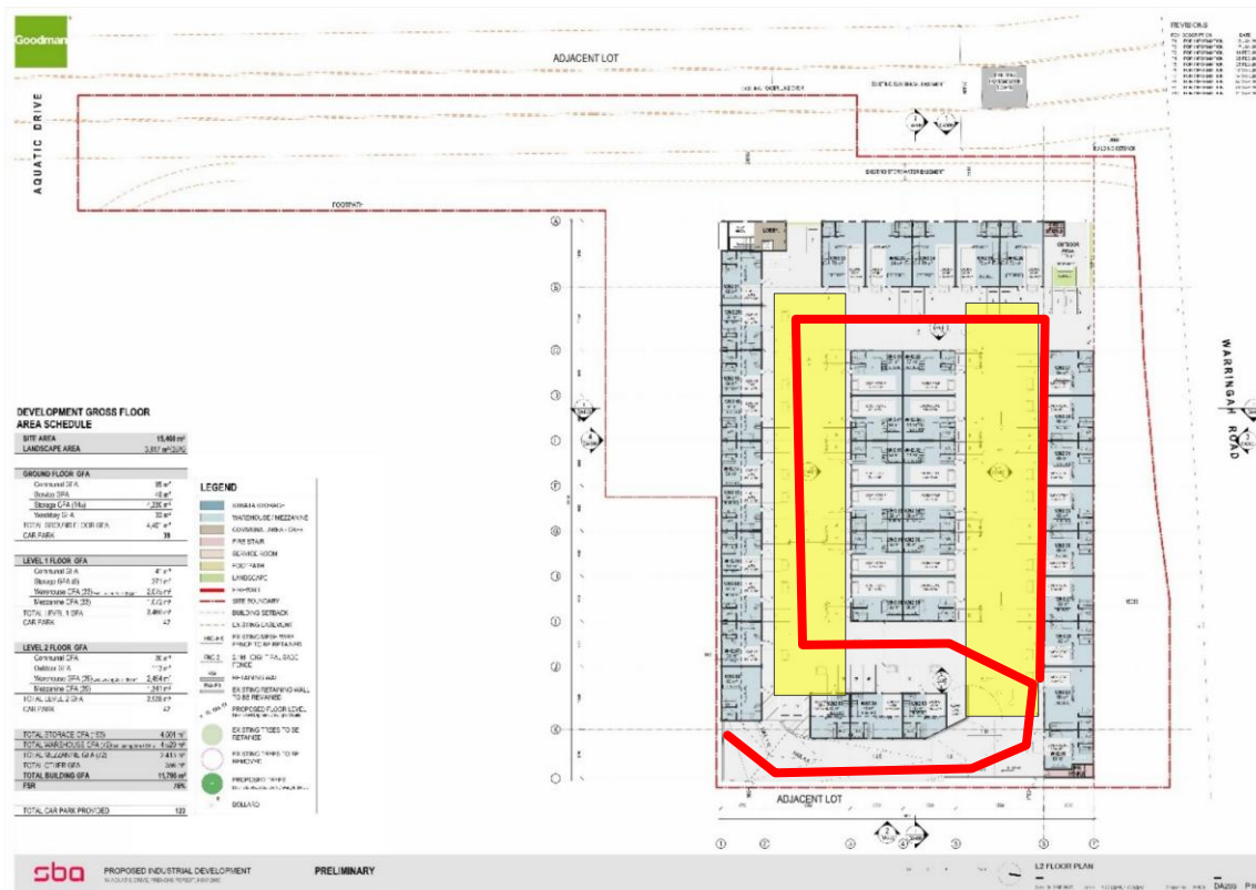
Figure 7 Heavy Vehicle Routes and Loading Areas – Level 2
