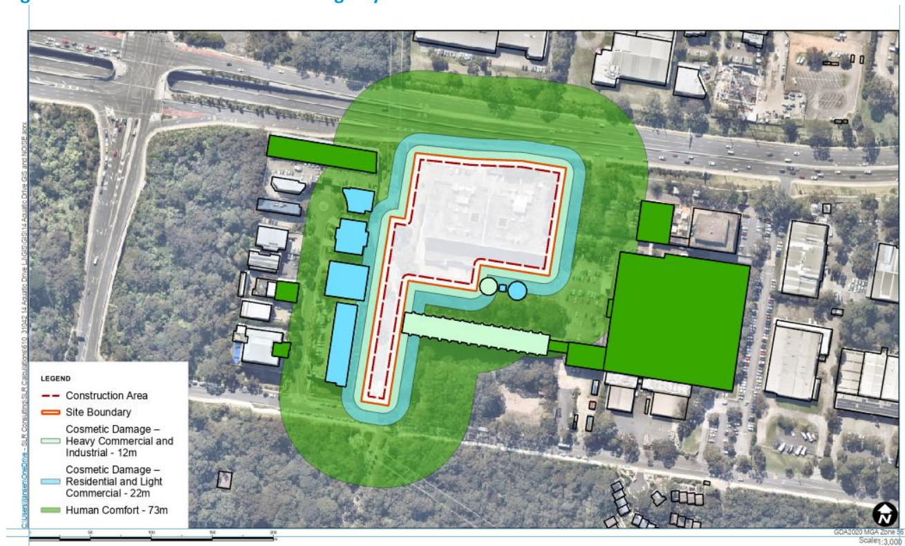
Figure 8 Construction Vibration – Large Hydraulic Hammer
