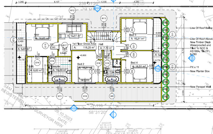
FIRST FLOOR 1:200
