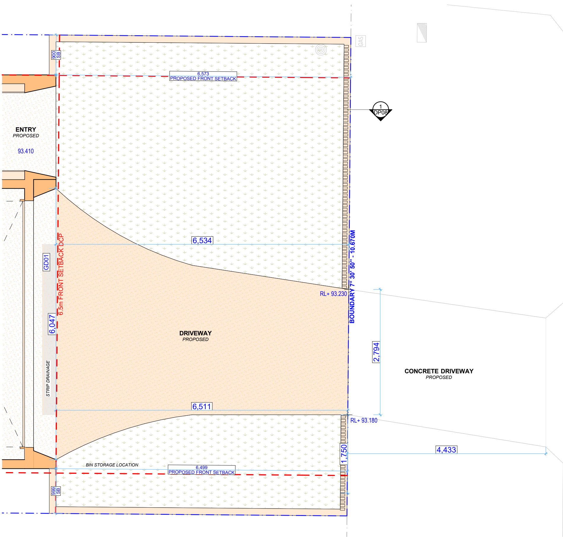
1 DRIVEWAY PLAN 1:50
