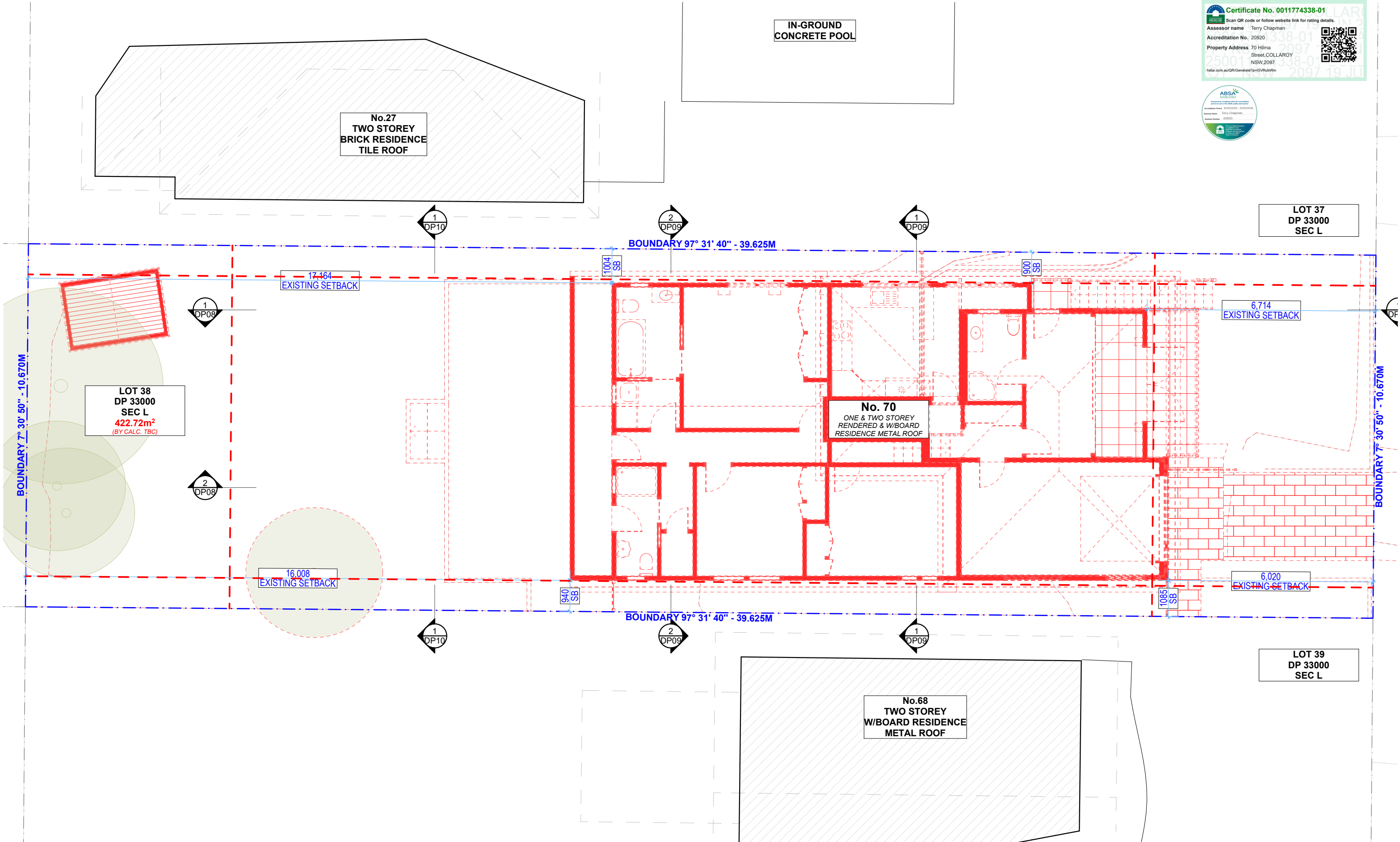
1 EXISTING HOUSE PLAN 1:100 NOTE: ALL DEMOLISHED ELEMENTS TO ENG. SPECIFICATIONS AND AS. 2601 - 2001
