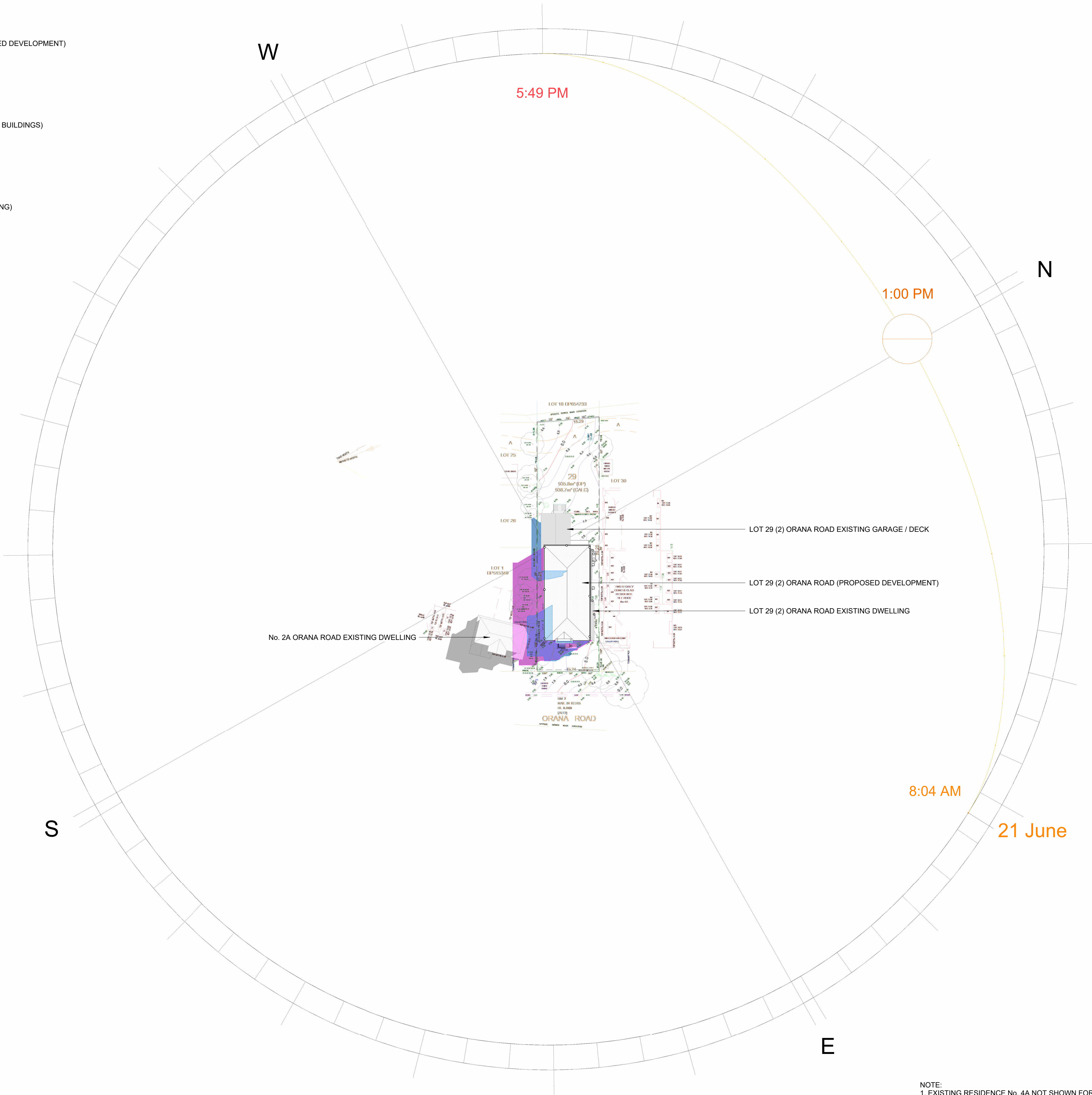
1pm 21ST JUNE SUN SHADOW DIAGRAM scale 1:500
