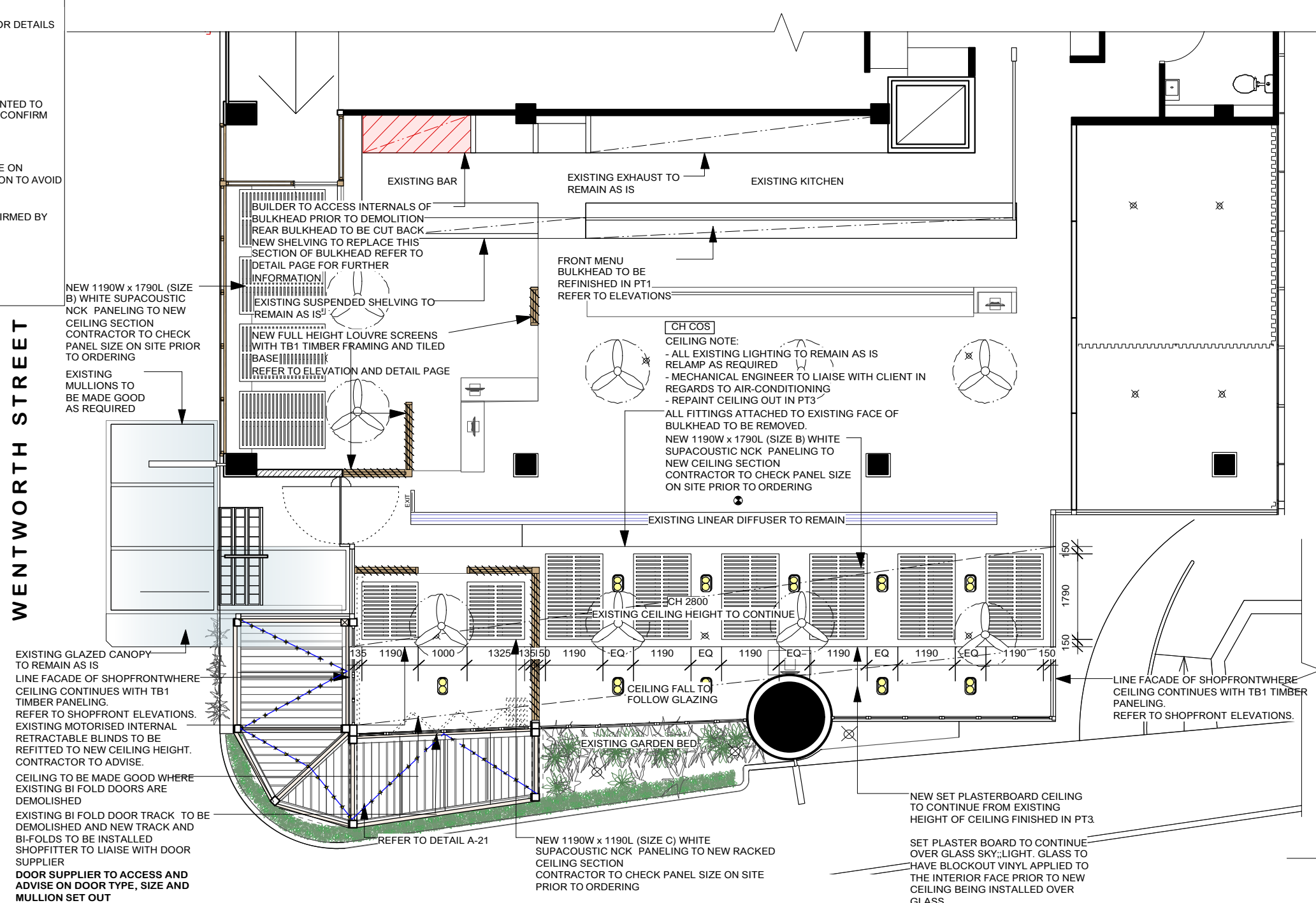
01 reflected ceiling plan Scale: 1:100
