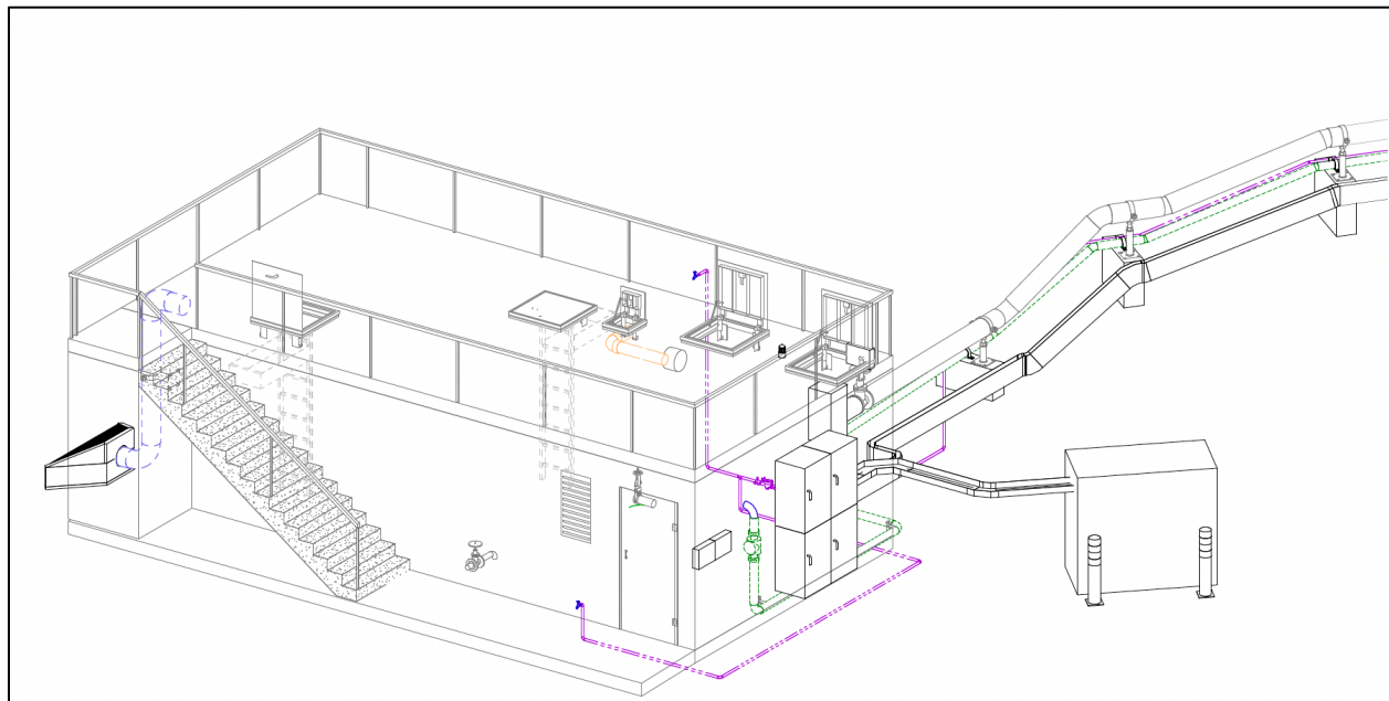
Figure 2 - Pump station layout
