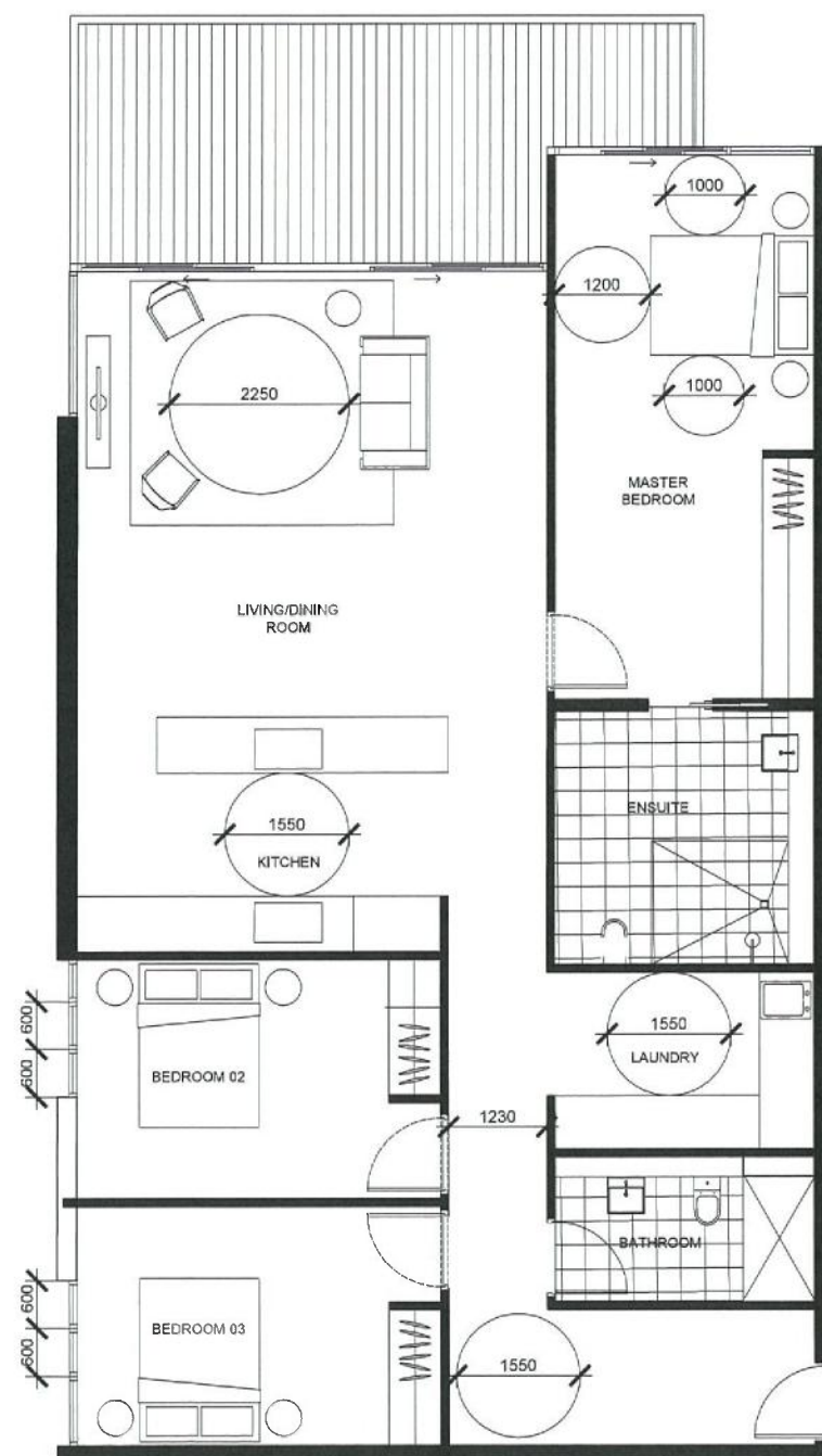
UNIT TYPE G 3BED - 145sqm UNITS: | 6.1.1 | 6.2.1 |
