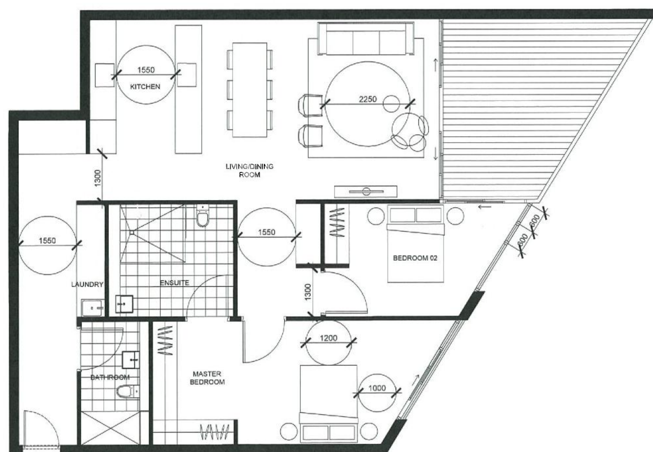
UNIT TYPE E 2BED - 124sqm UNITS : | 1.1.2 |
