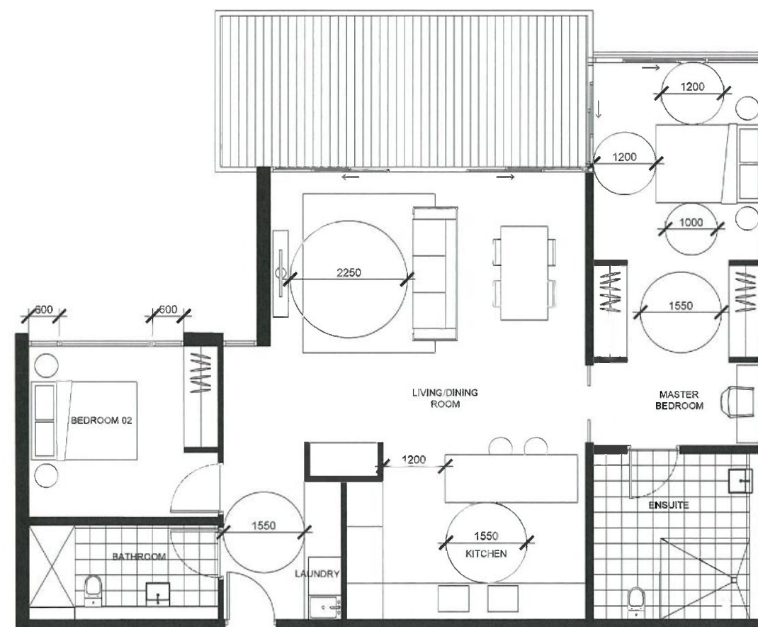
UNIT TYPE H 2BED - 112sqm UNITS: | 1.1.4 | 1.2.7 |
