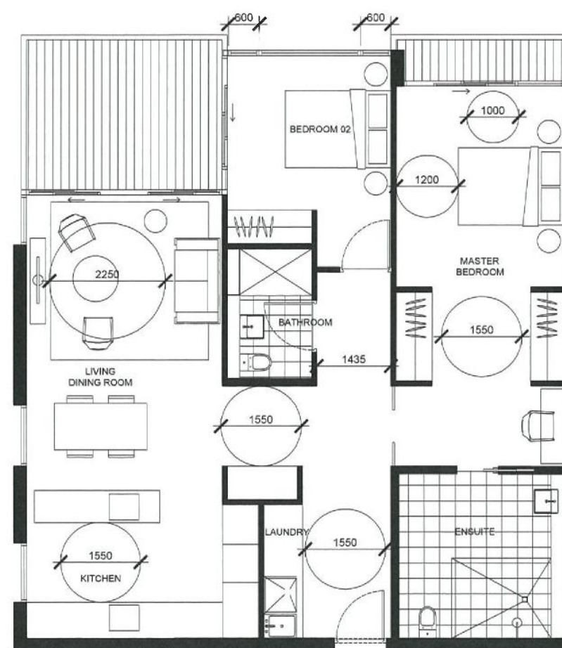
UNIT TYPE D 2BED - 104sqm
