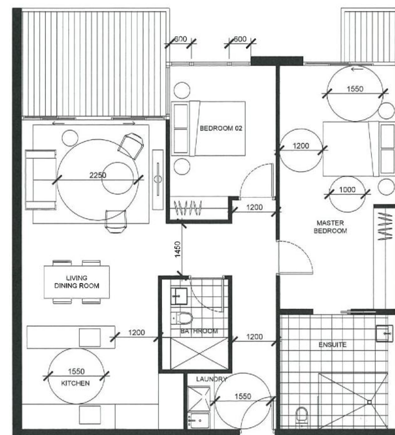
UNIT TYPE J 2BED - 99sqm UNITS: | 1.2.6 |
