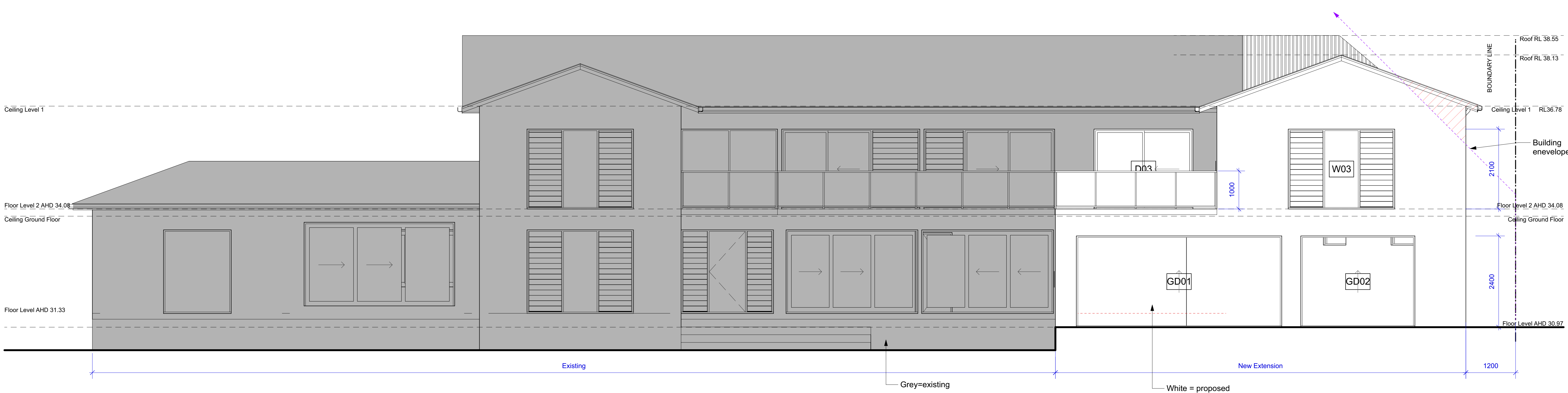
Elevation - South East (Front) 1:50@A1 1:100@A3. Do not scale off plan
