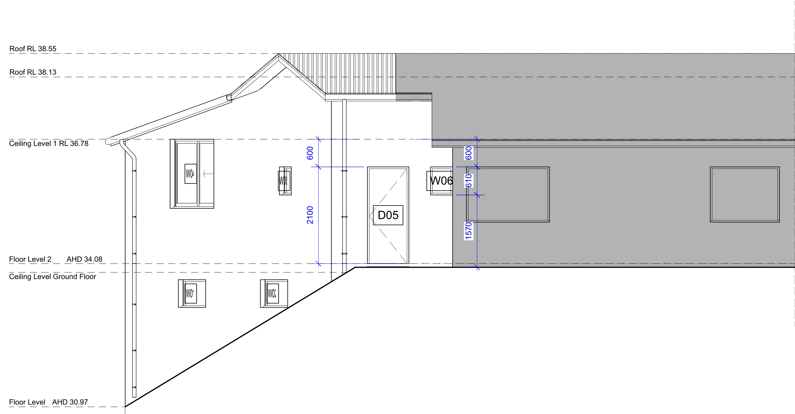
Elevation - South West (Rear) 1:50@A1 1:100@A3. Do not scale off plan
