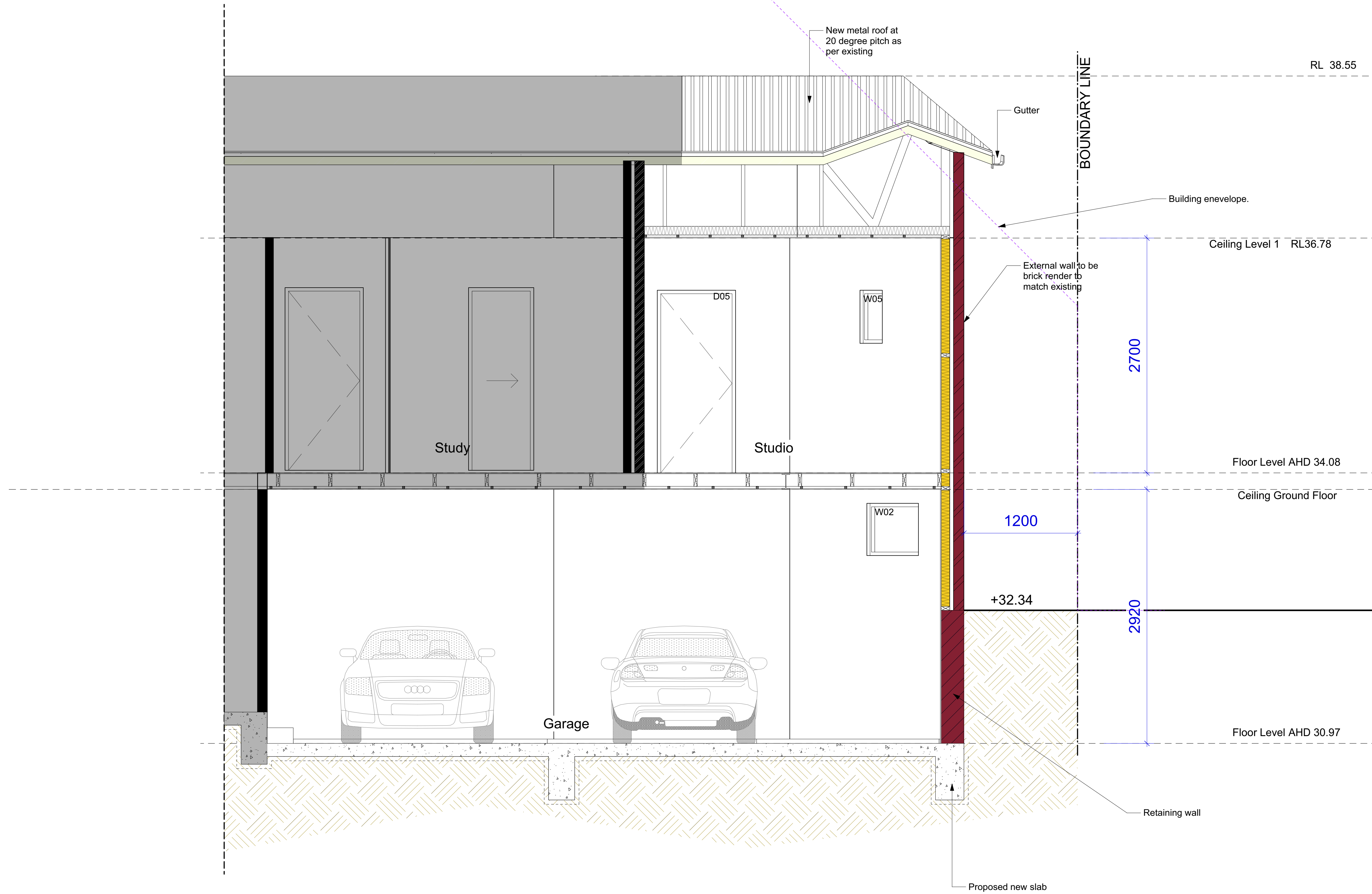
Section B 1:25@A1 1:50@A3. Do not scale off plan
