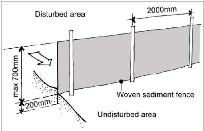
Sedimentation Control Fence Not to scale.
