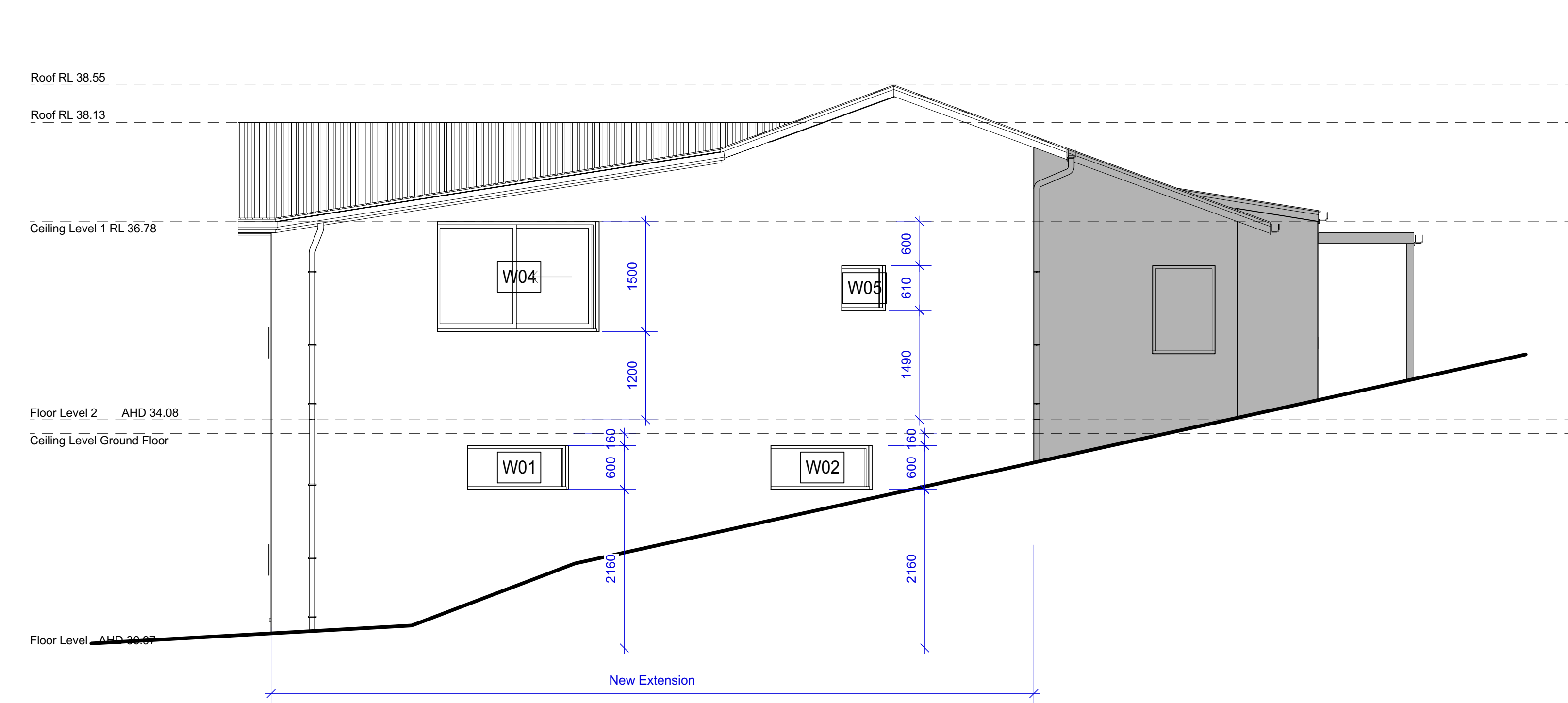
Elevation - North East (Side) 1:50@A1 1:100@A3. Do not scale off plan
