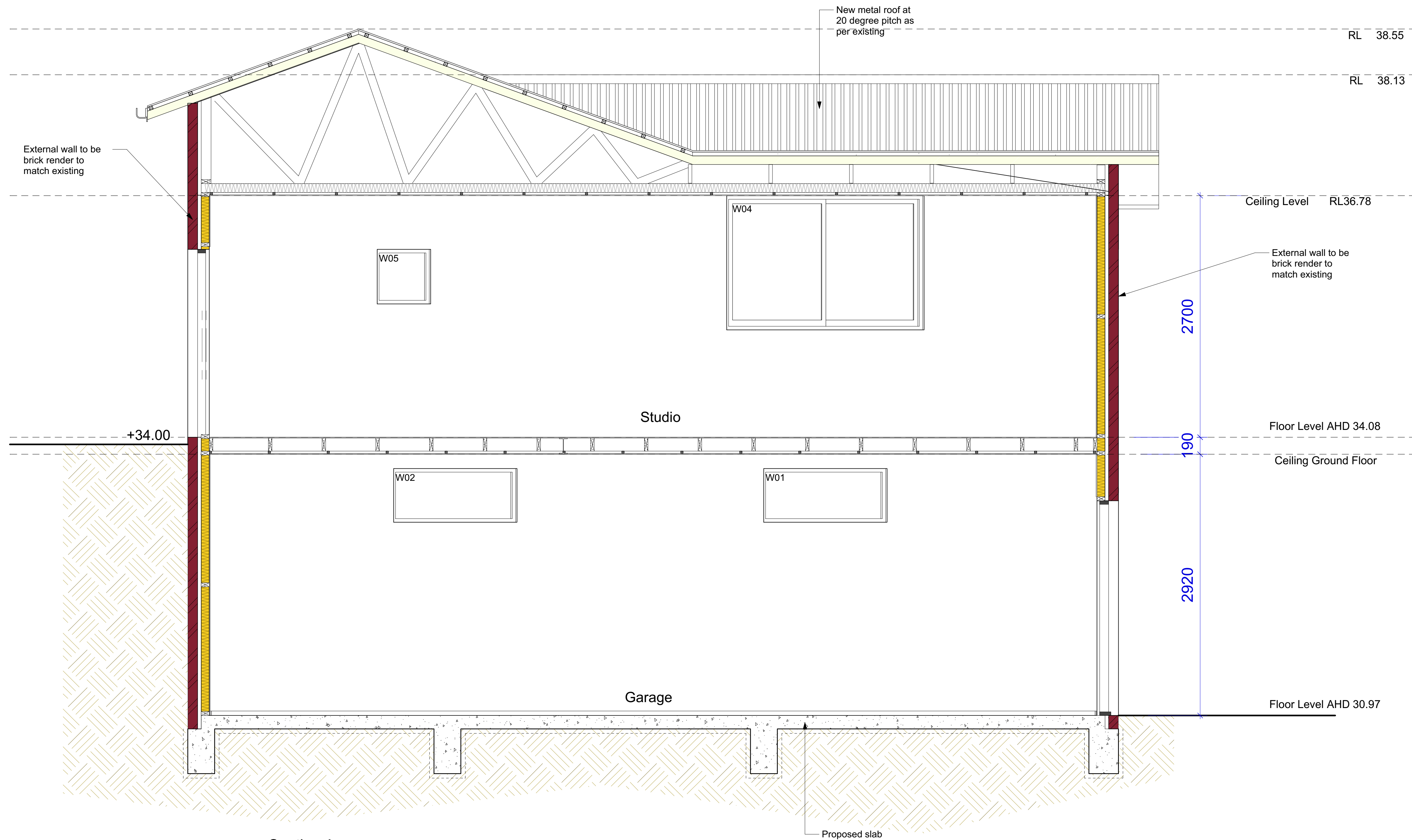
Section A 1:25@A1 1:50@A3. Do not scale off plan
