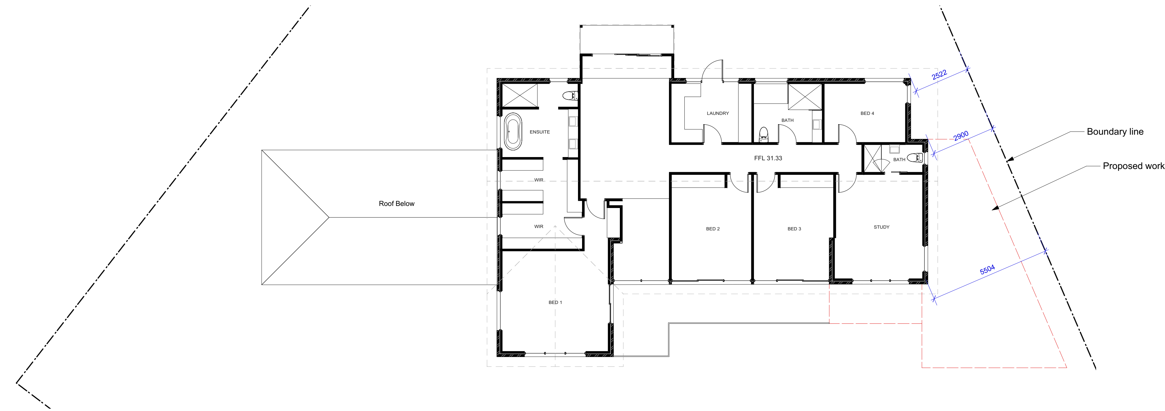
Existing First Floor Plan 1:50@A1 1:100@A3. Do not scale off plan
