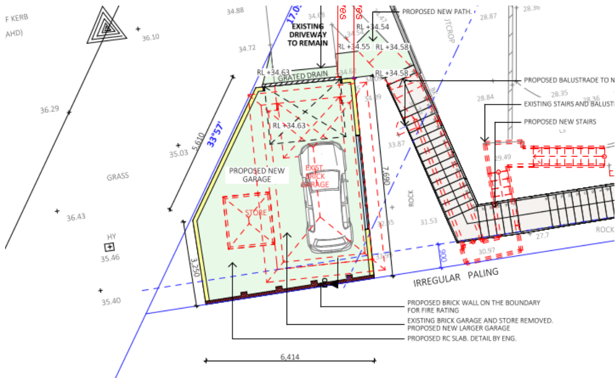
Figure 1: Side setback non-compliance.
