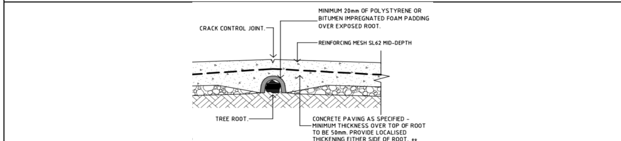
Image D: Example method for bridging concrete surfacing over tree roots provided in the Canterbury Bankstown Council standard drawings. 7
