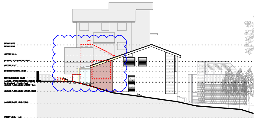
2 North Elevation NTS
