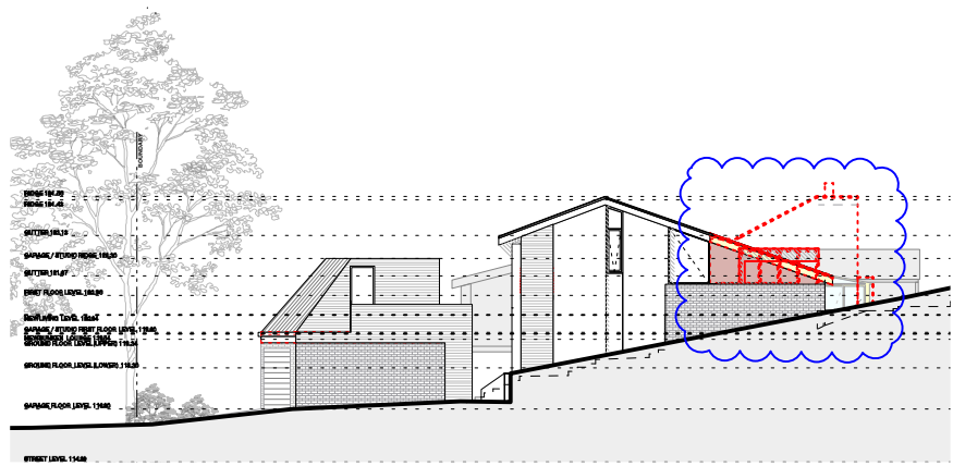
4 South Elevation NTS
