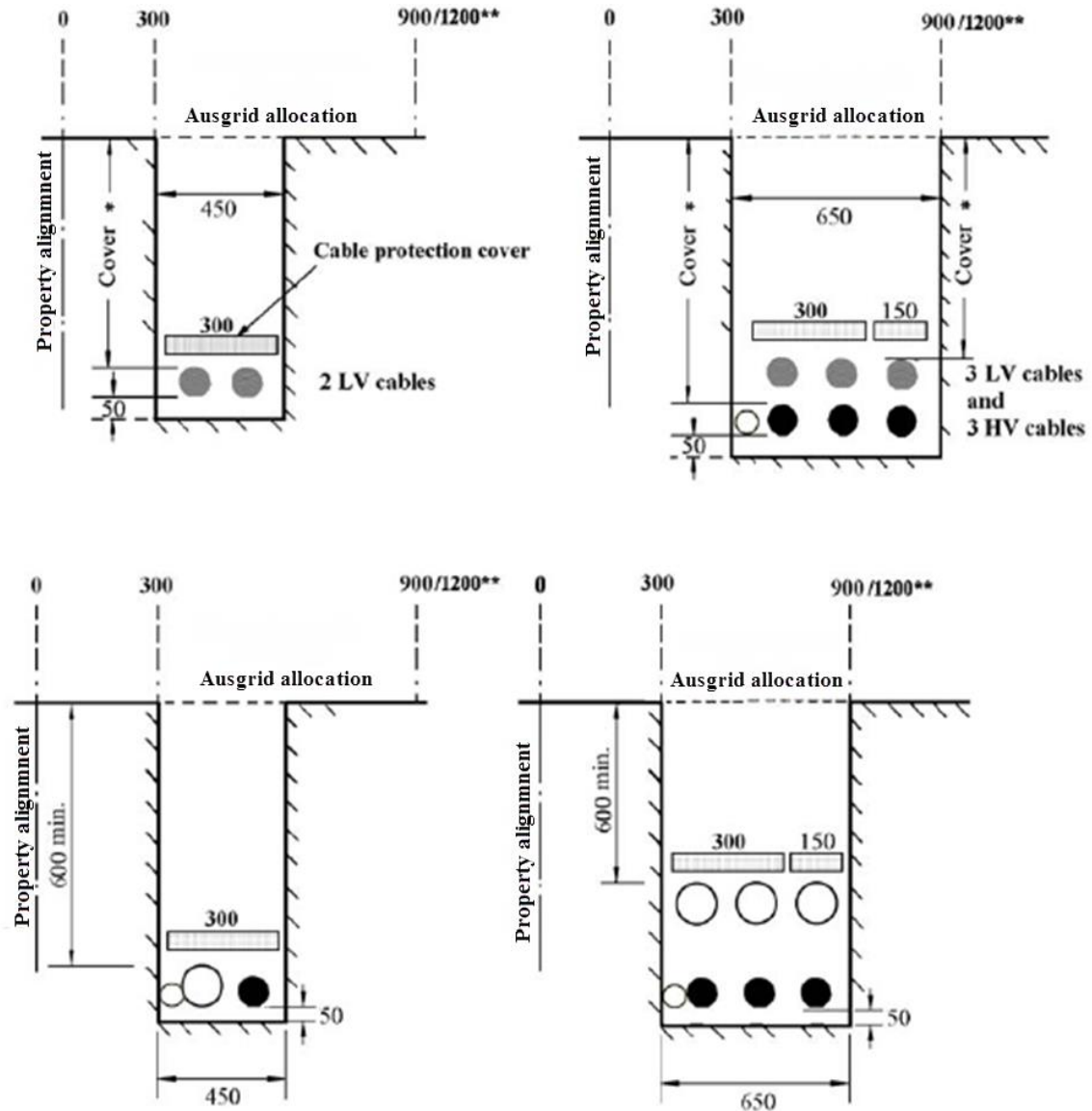
Figure 20 – Typical trench layout
