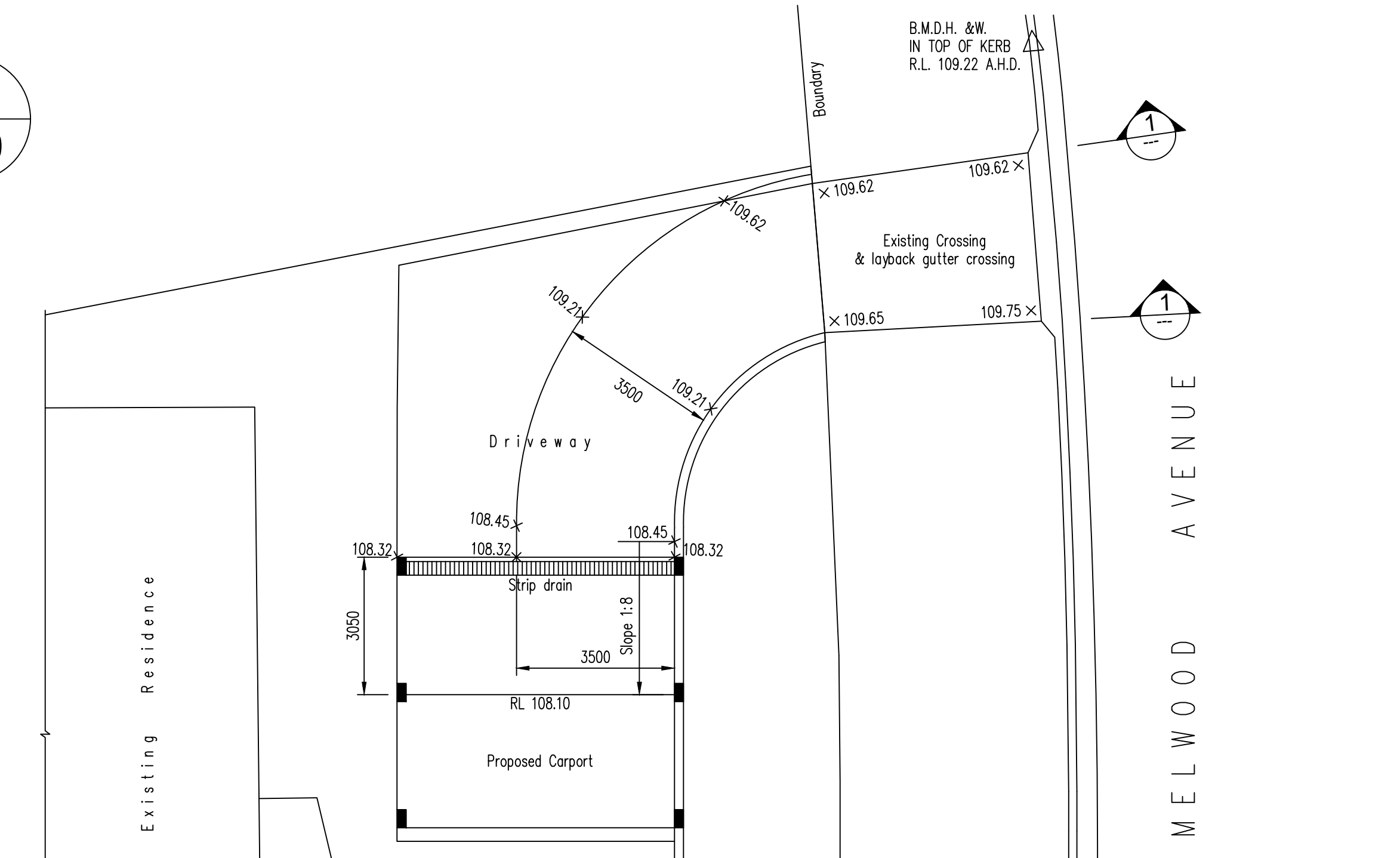
PLAN ON CARPORT AND DRIVEWAY
