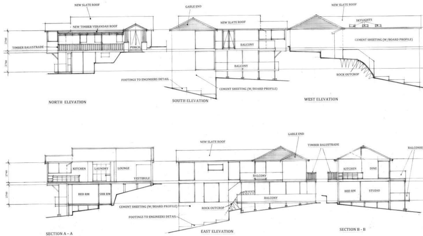
PROPOSED ALTERATIONS & ADDITIONS TO COTTAGE AT 1 KANIMBLA CRES. BILGOLA PLATEAU FOR JOHN & HELEN WOOD SCALE: 1:100 (AT A2) DATE: 17 APRIL 2021 DRAWING NO. 6818/502
