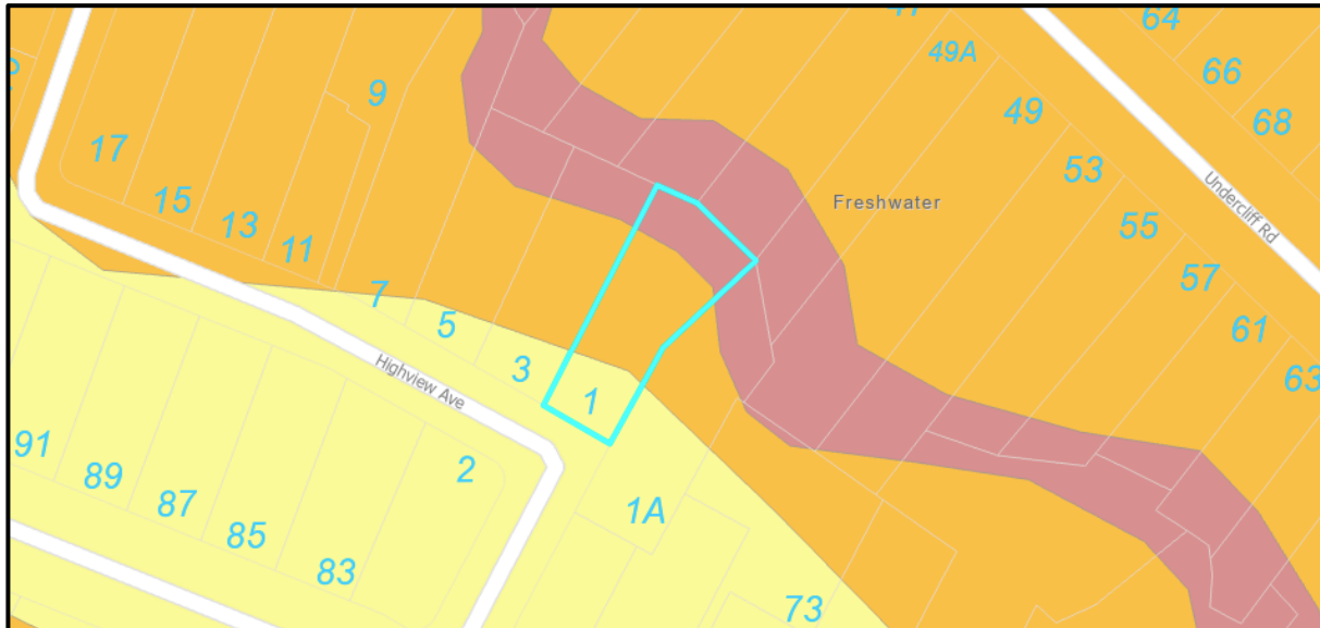
Figure 1. Warringah Landslip Risk Map: 1 Highview Avenue, Queenscliff NSW (© NBC Maps)
