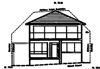
EAST ELEVATION Front
