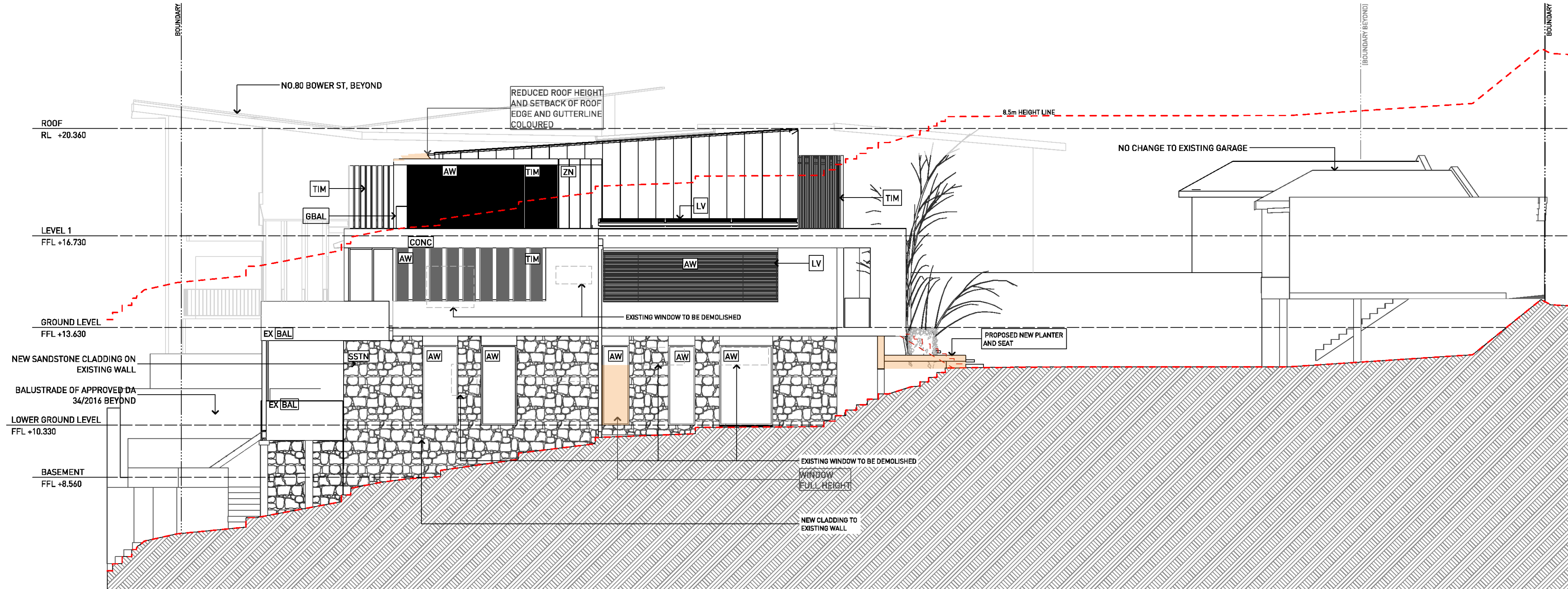
4 WEST ELEVATION 1:100
