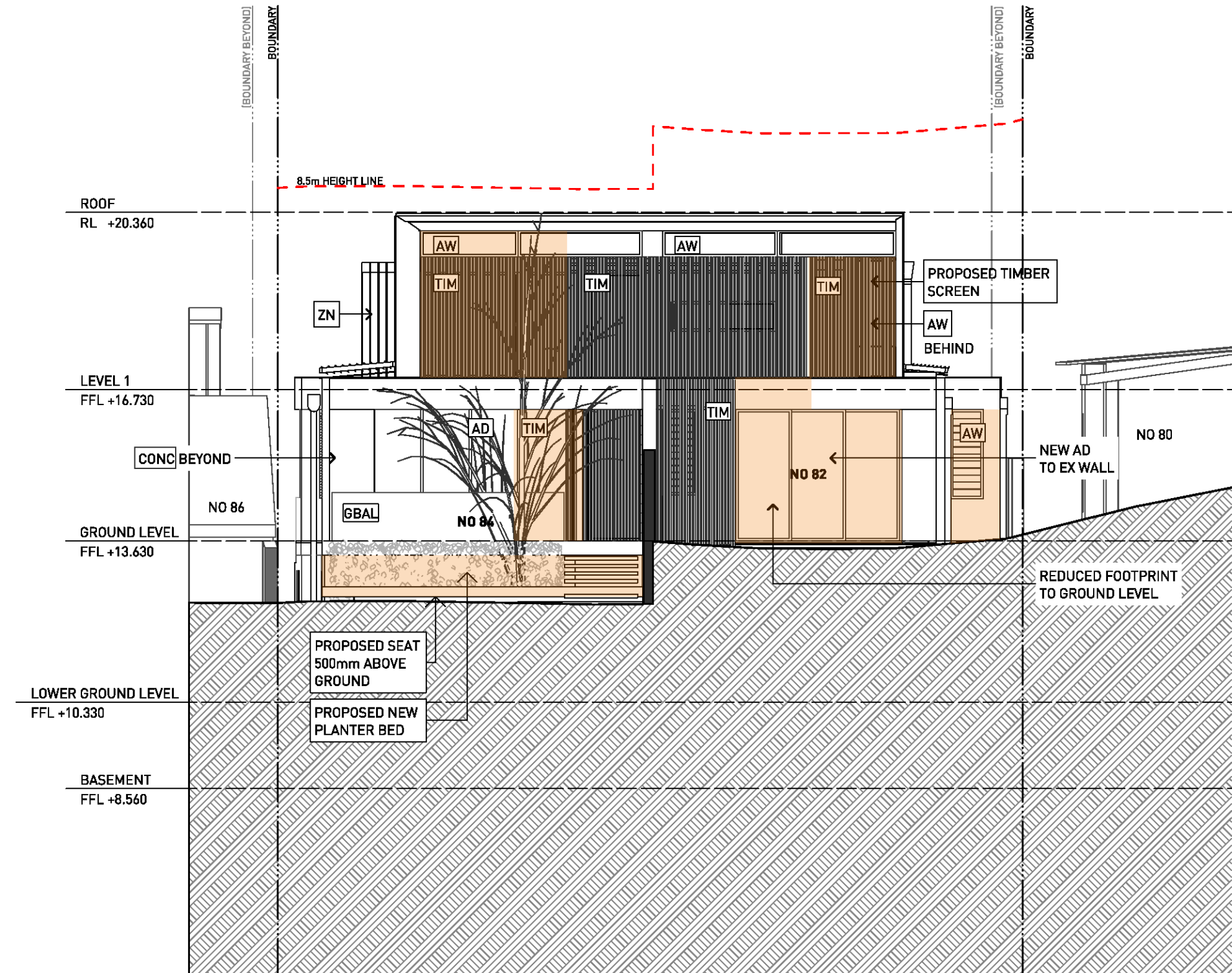
3 SOUTH ELEVATION 1:100
