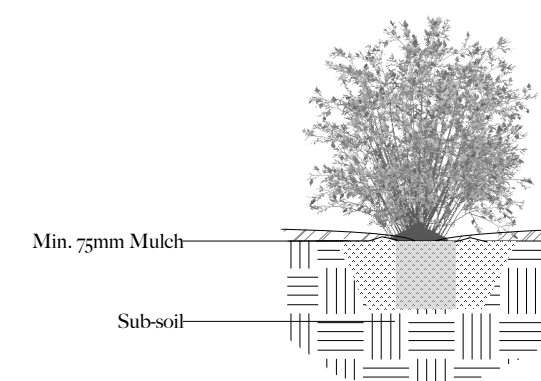
Typical Shrubs/Grass Planting in a Garden Bed NOT TO SCALE
