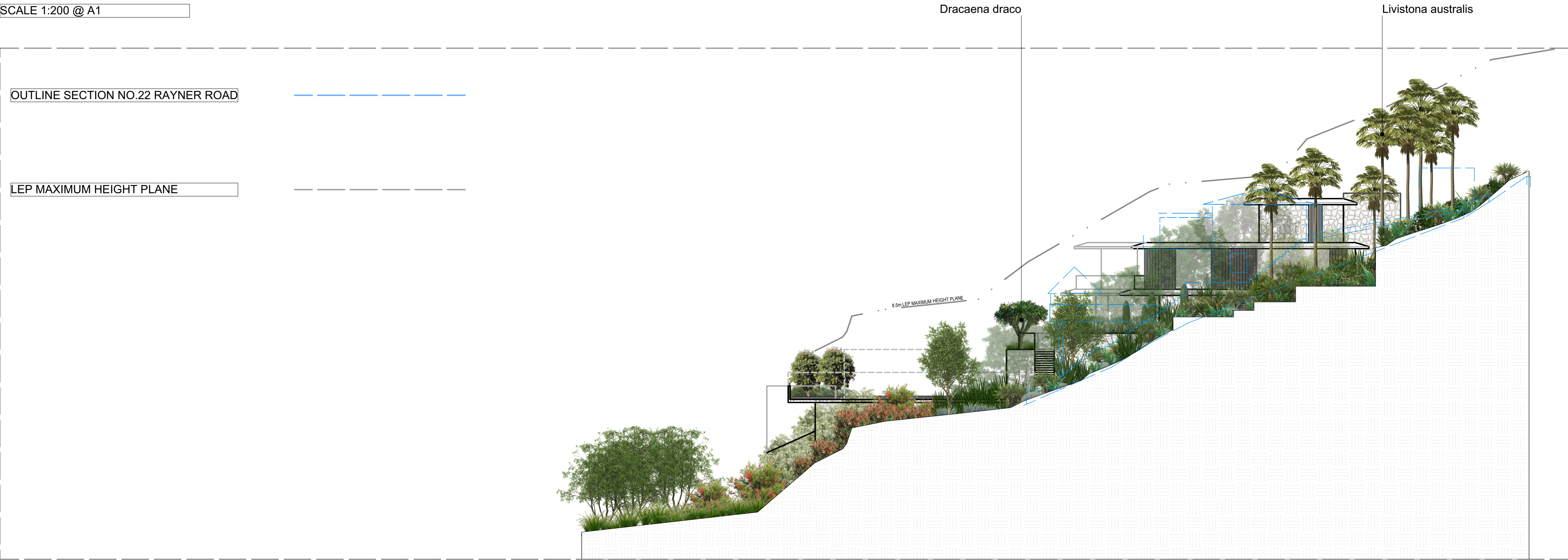
ELEVATION B VIEW FROM NO.30 RAYNER ROAD
