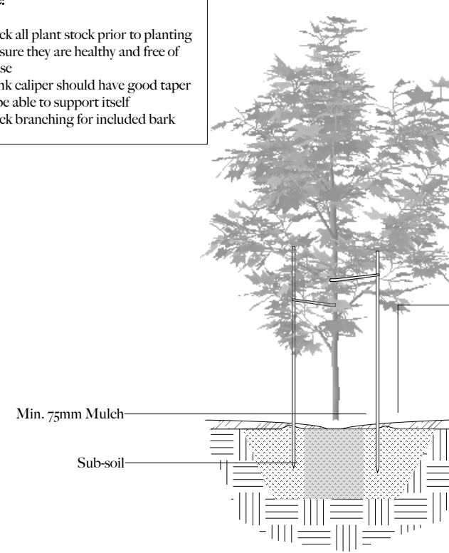
Typical Tree Planting in a Garden Bed NOT TO SCALE
