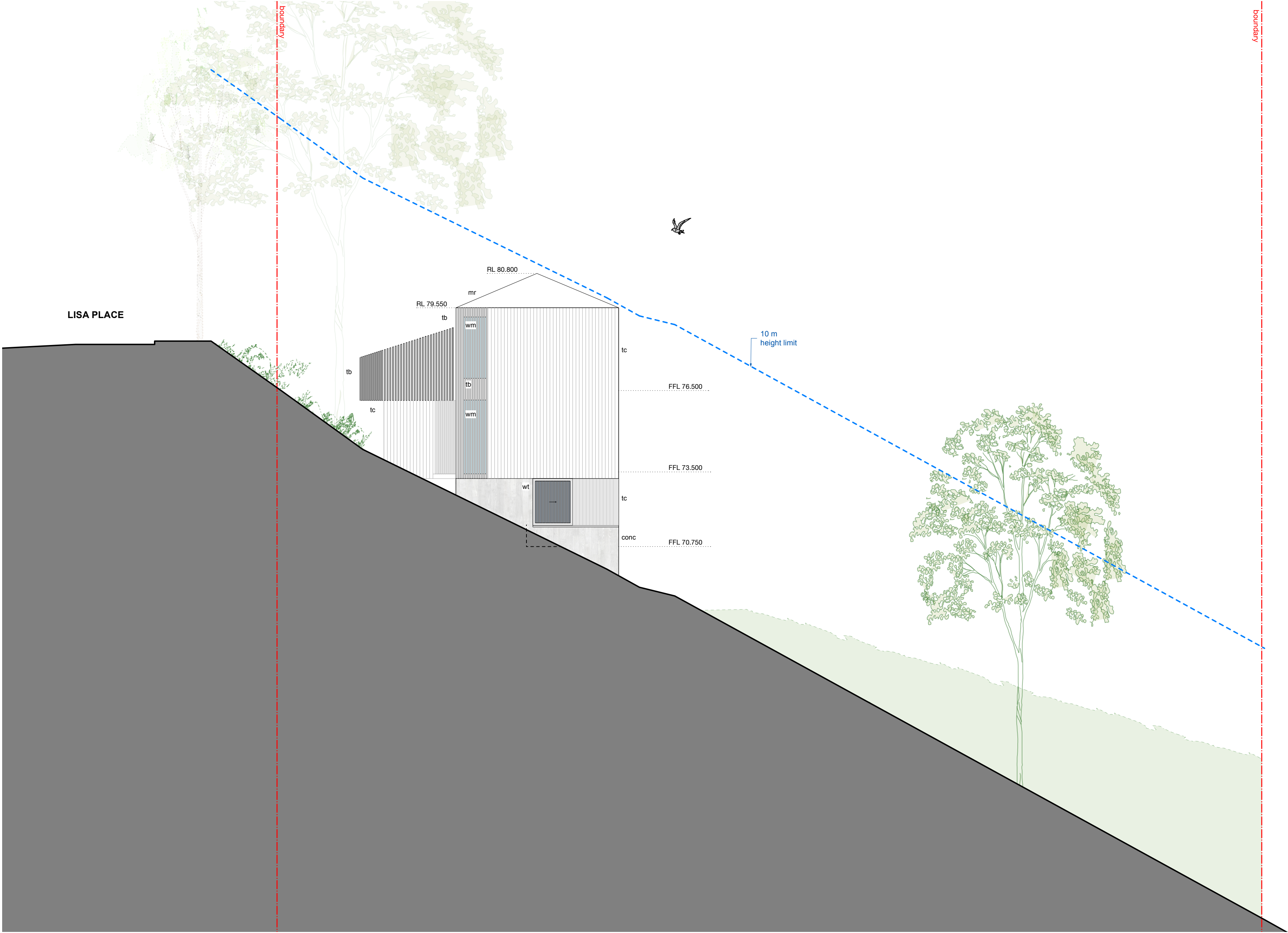
north-west elevation
