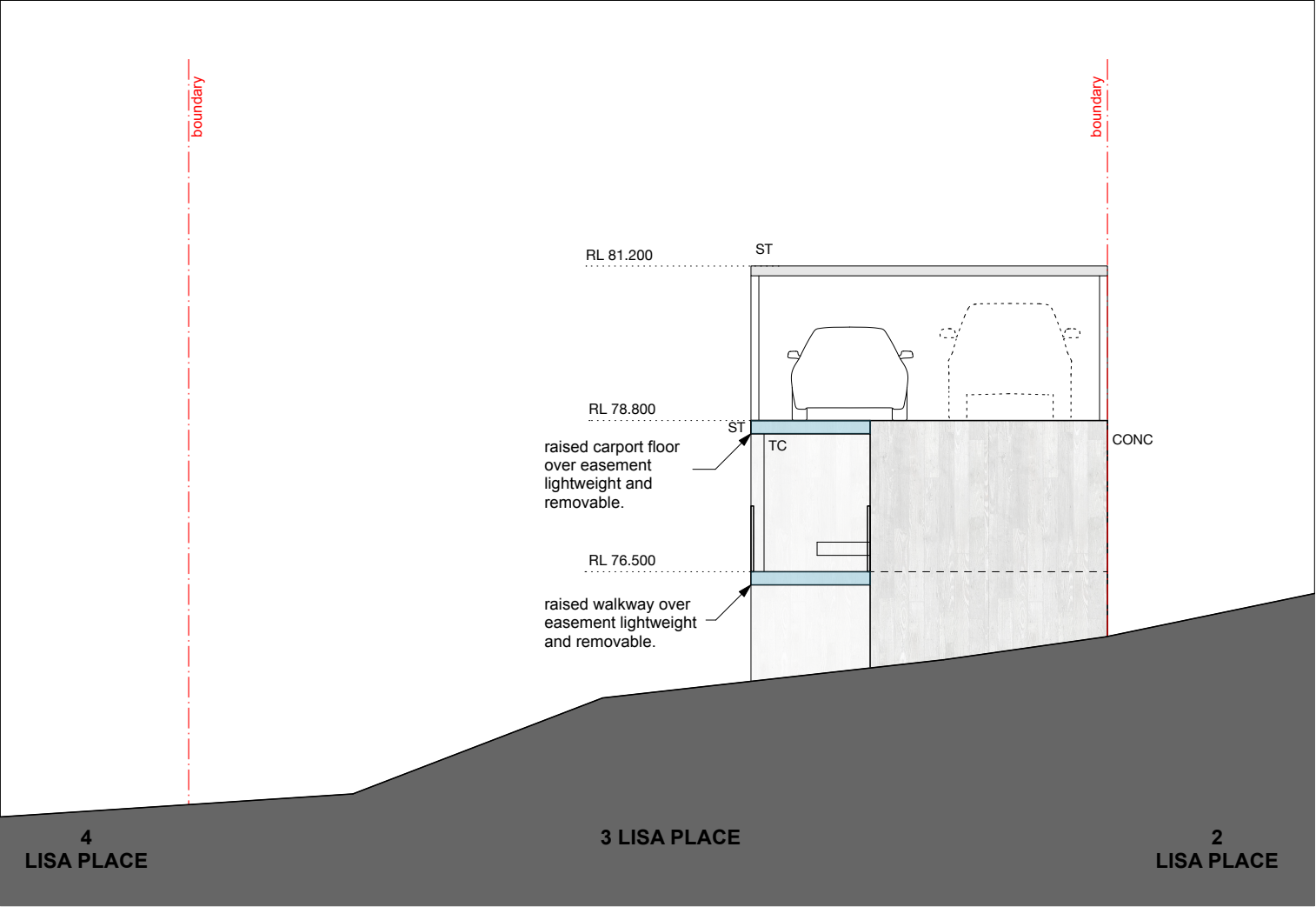
west elevation
