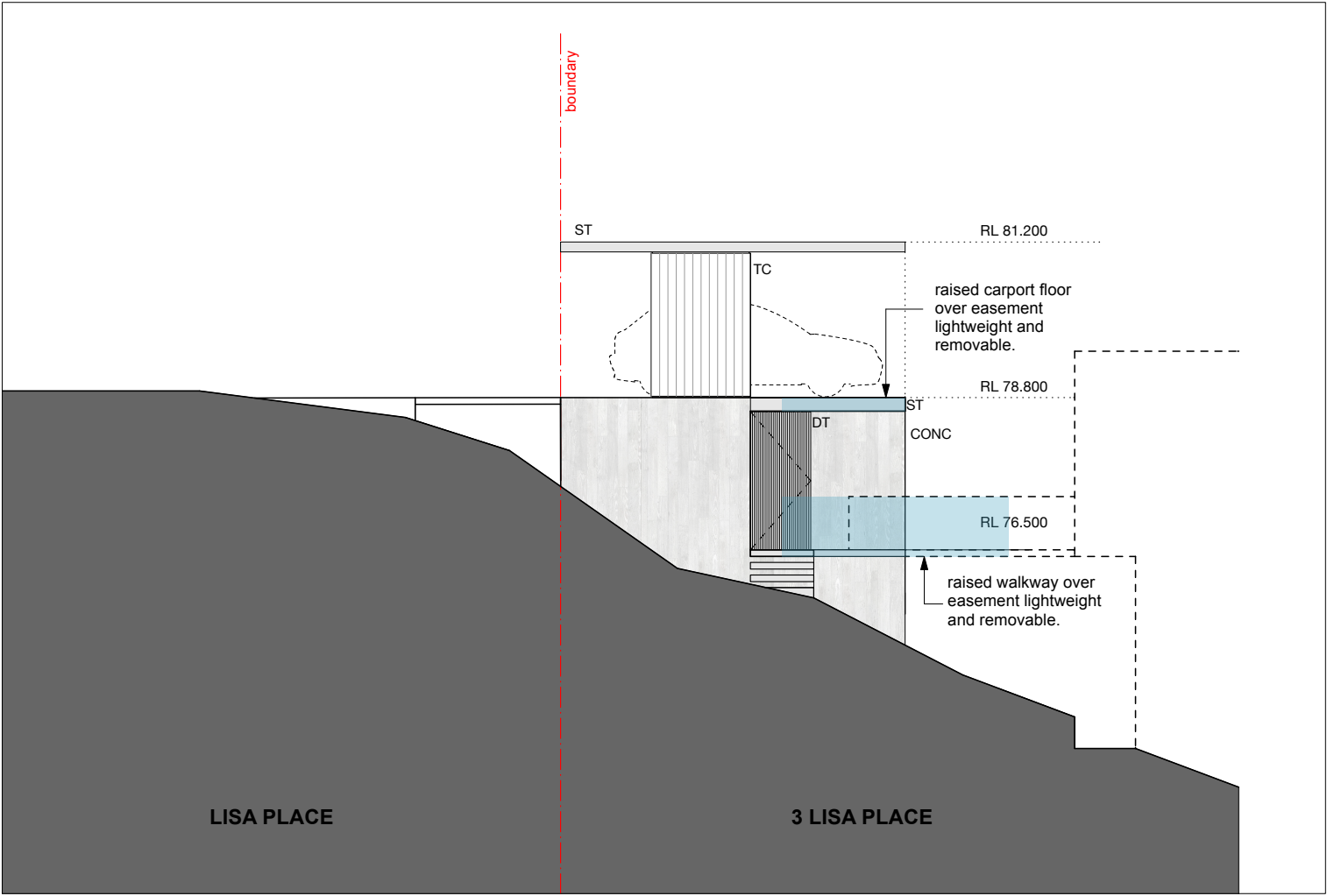
north elevation
