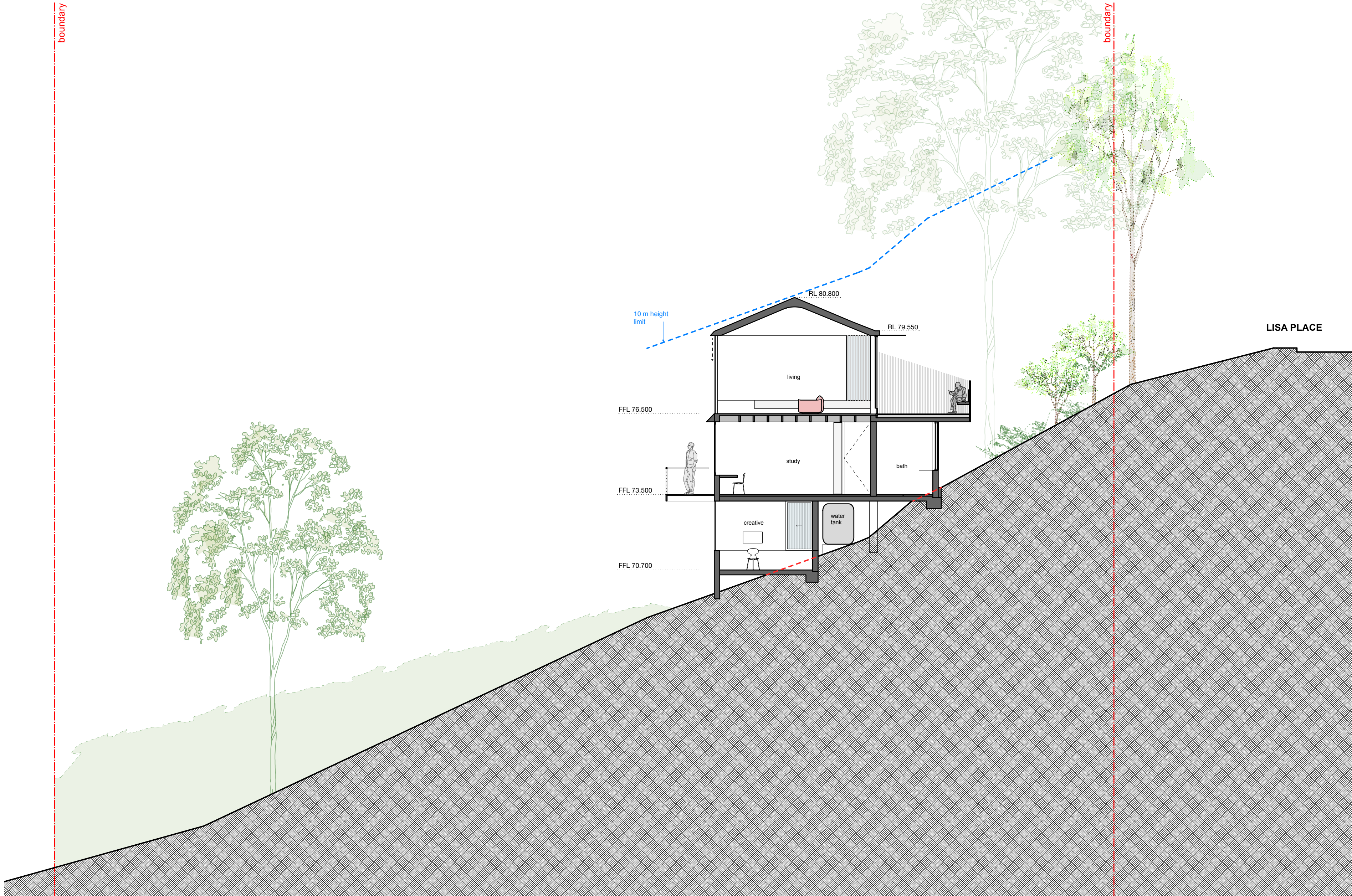
section a
