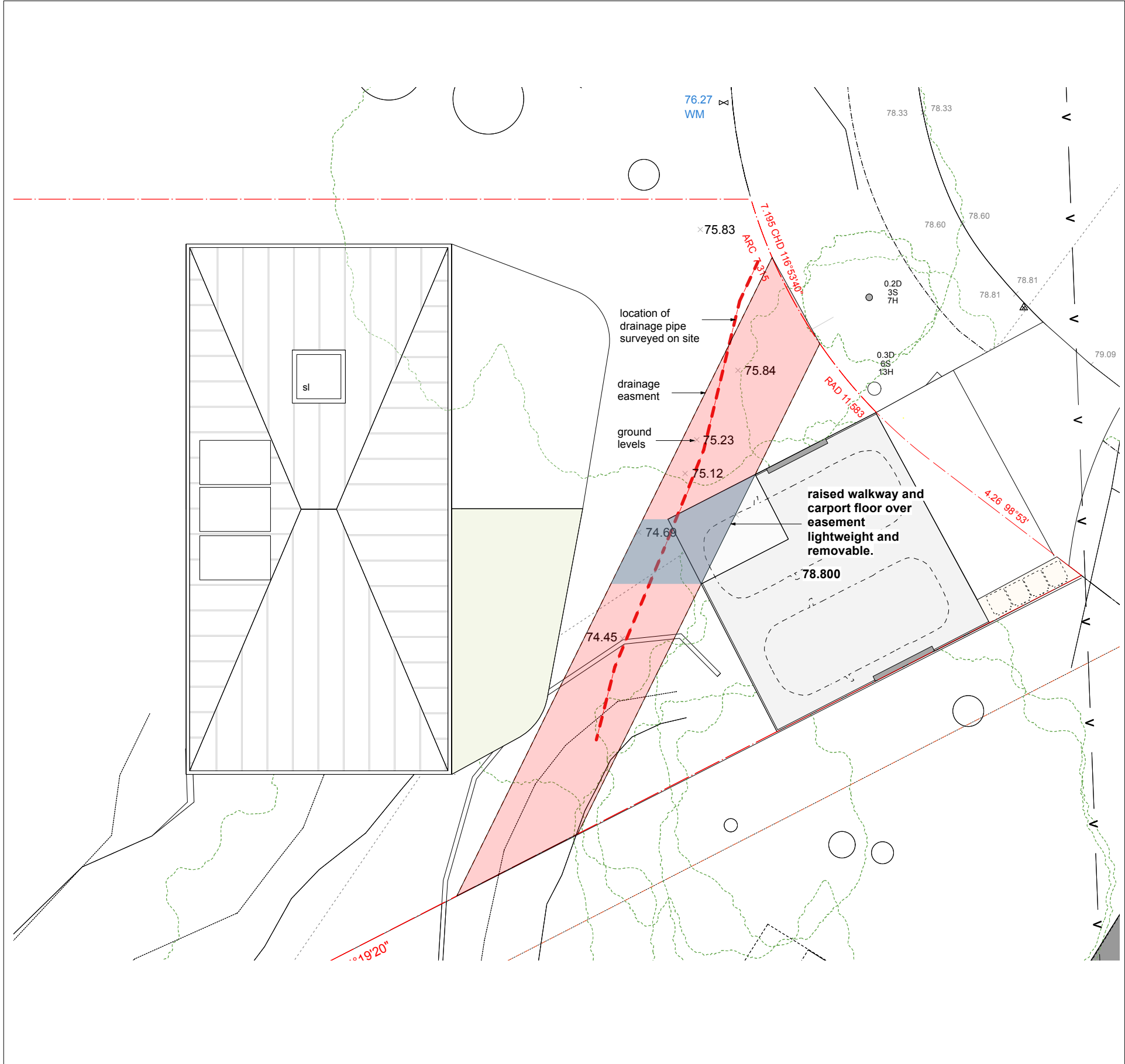
location of stormwater pipe
