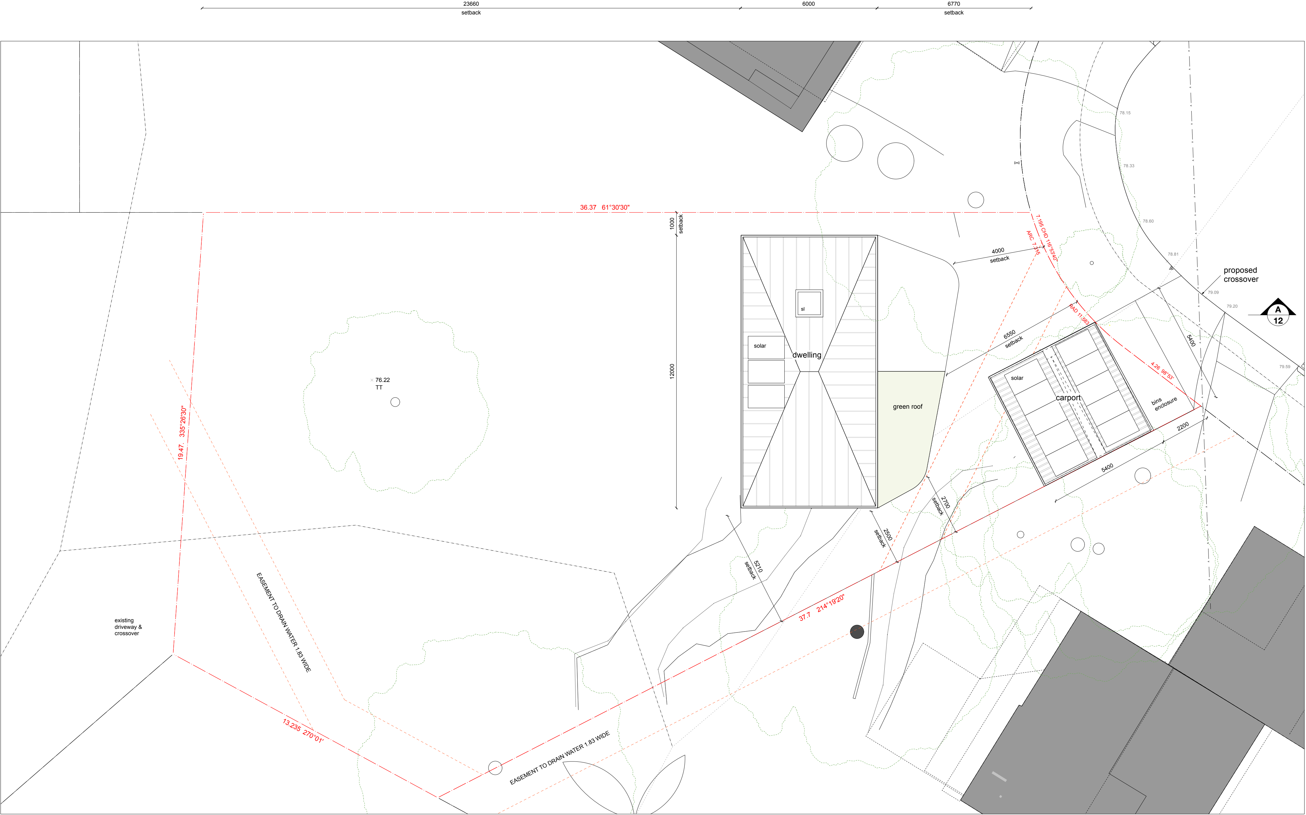
roof plan
