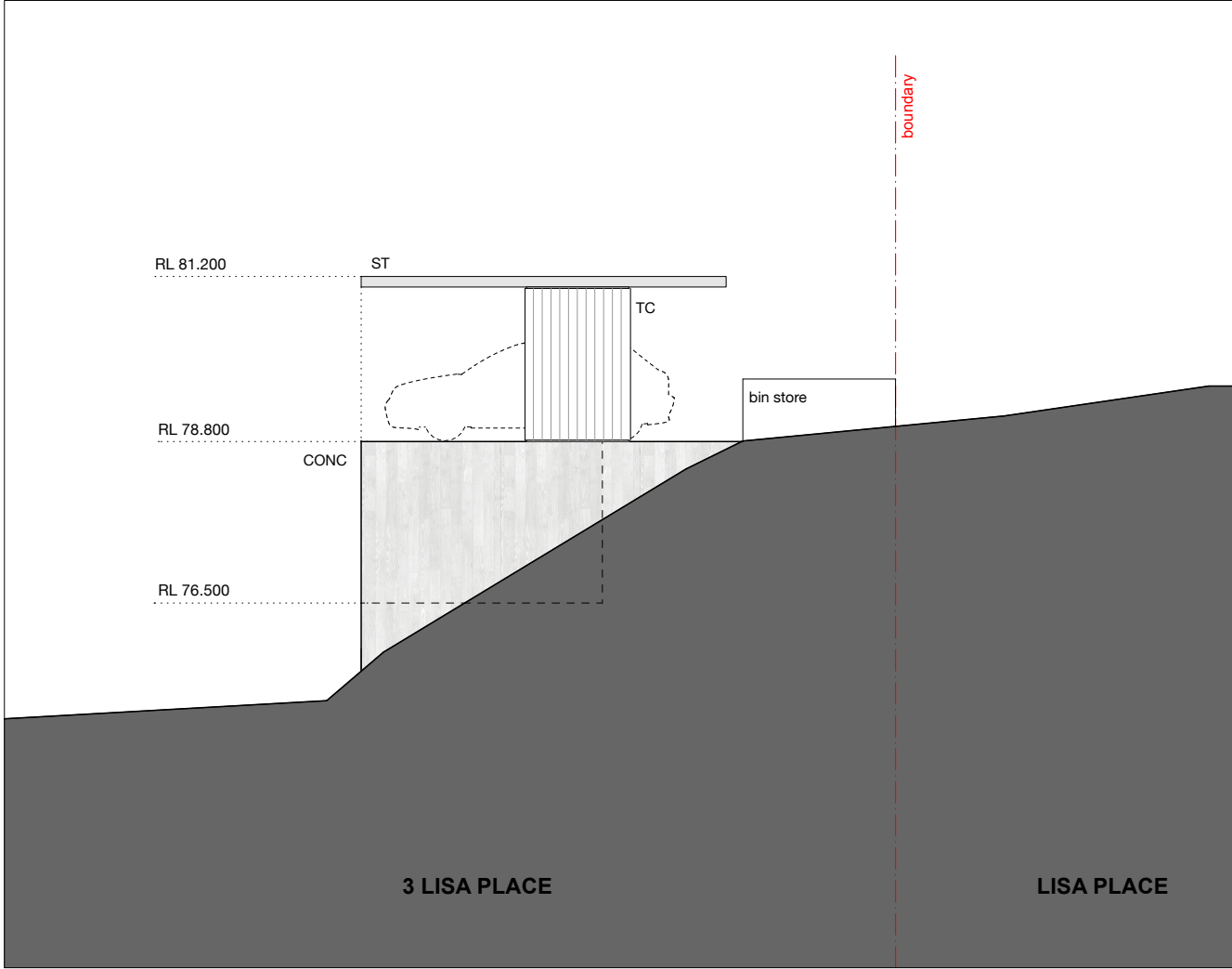
south elevation
