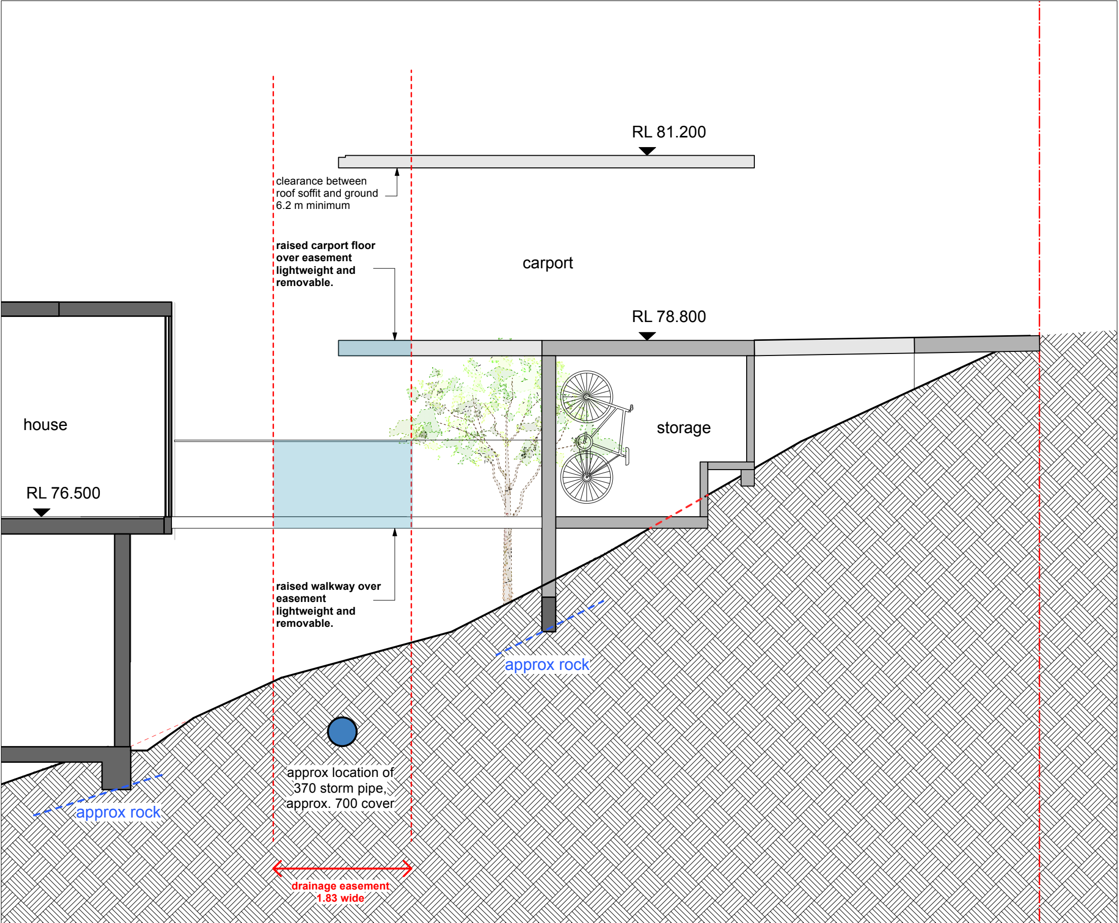
section @ easment
