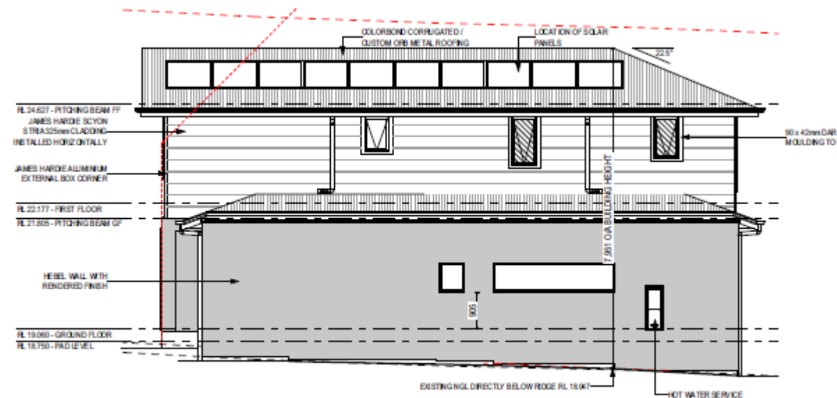
RIGHT ELEVATION (NORTH-WEST) SCALE: 1:100
