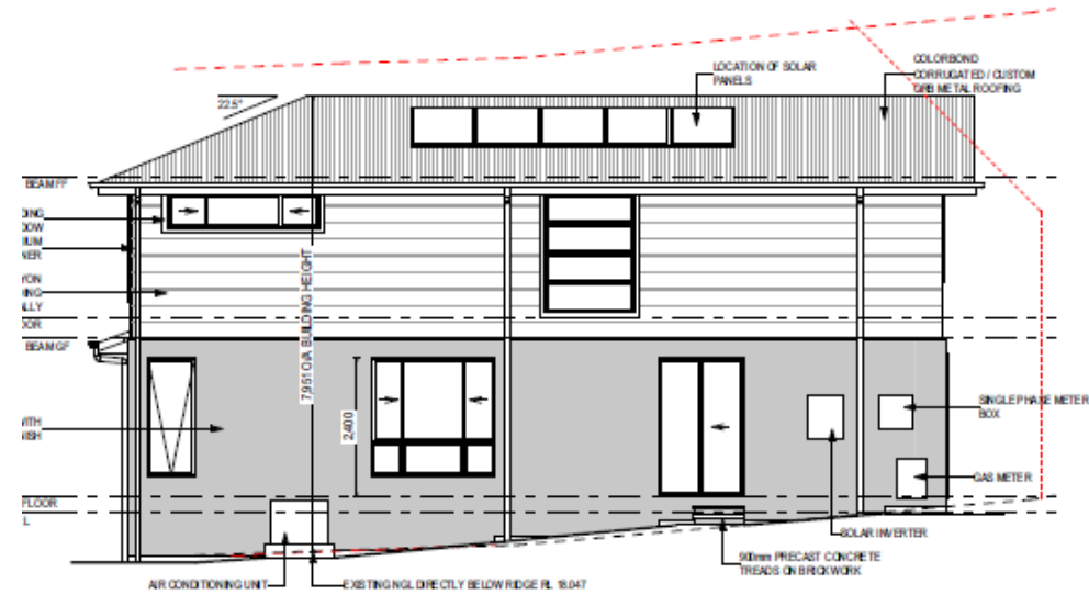
LEFT ELEVATION (SOUTH-EAST) SCALE: 1:100
