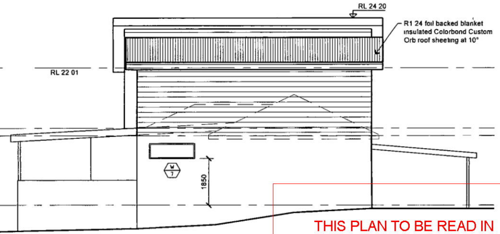
WEST ELEVATION
