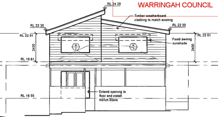
NORTH ELEVATION
