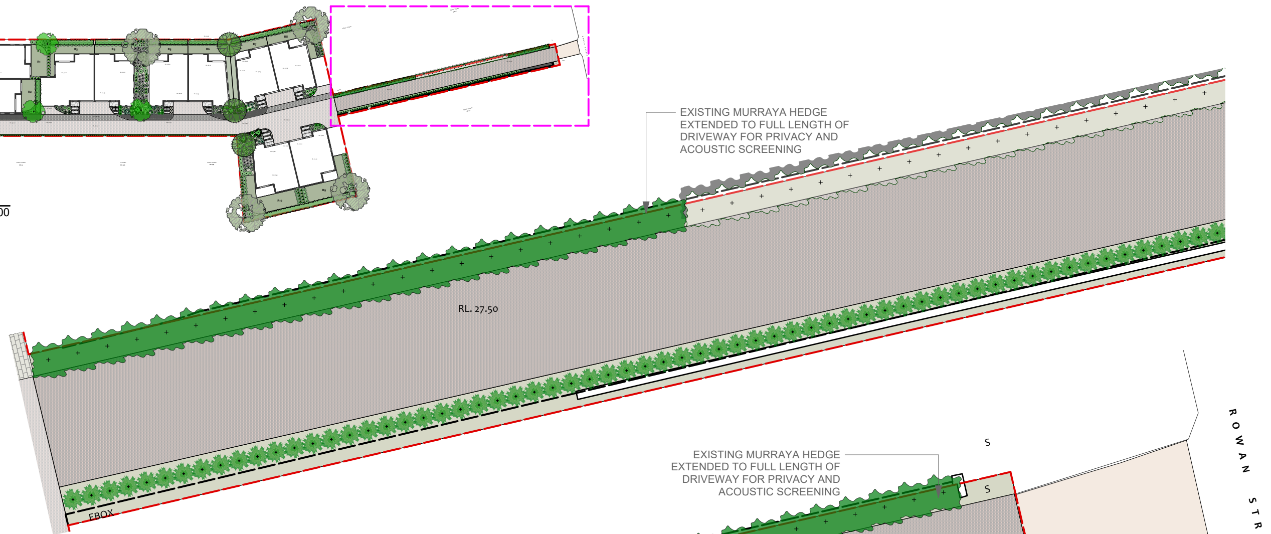
1 DRIVEWAY-1 Scale: 1:100
