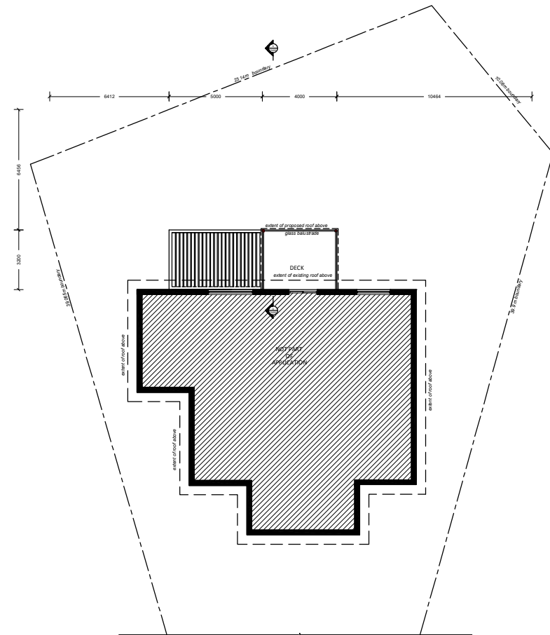
PROPOSED FIRST FLOOR PLAN SCALE: 1:200
