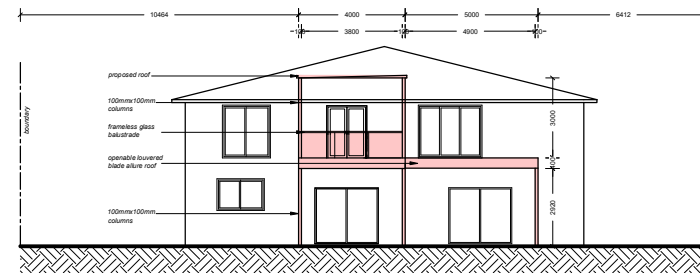
PROPOSED NORTH ELEVATION SCALE: 1:200
