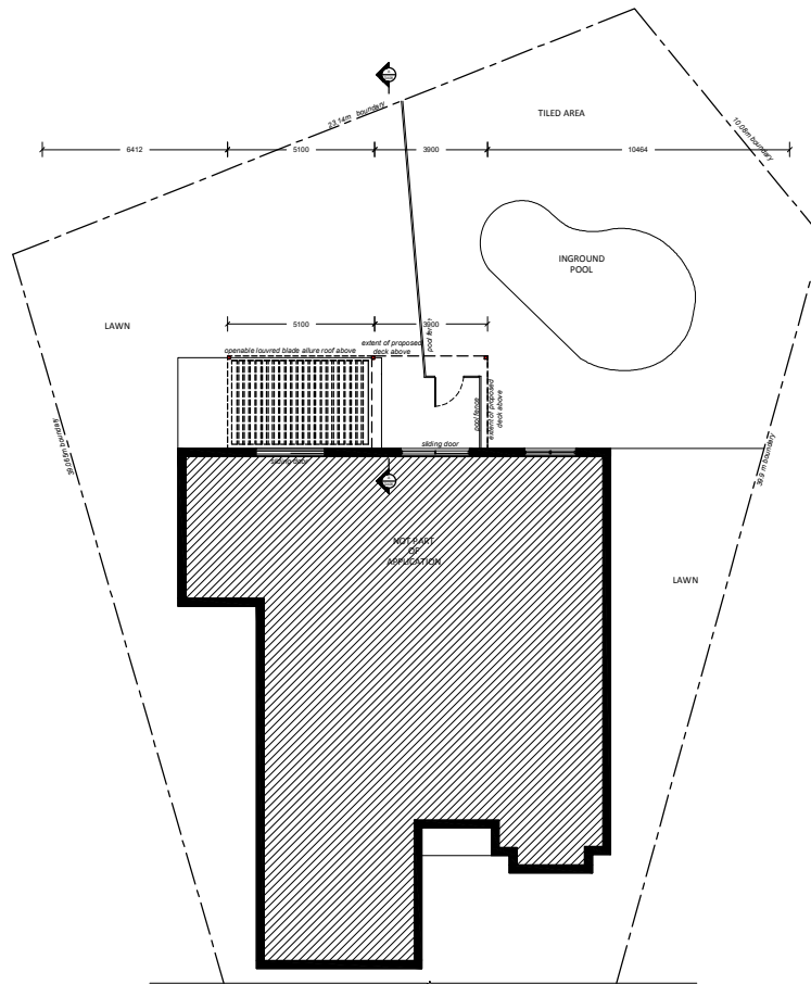
PROPOSED GROUND FLOOR PLAN SCALE: 1:200
