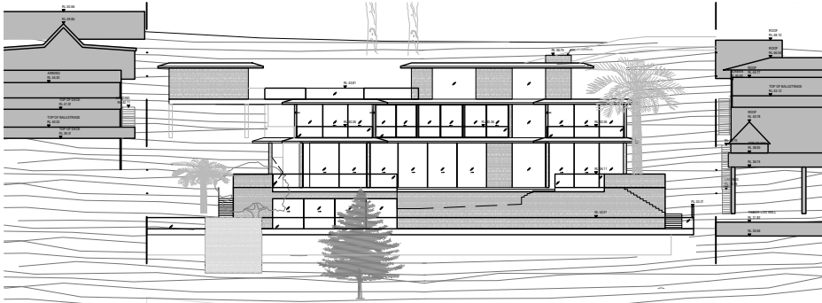
2 NORTH ELEVATION 1:600 @ A4
